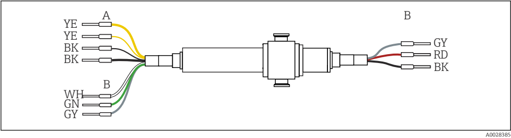
3 OUSAF44 connecting cable A Light source (lamp) power supply B Signals of measurement and reference detector
