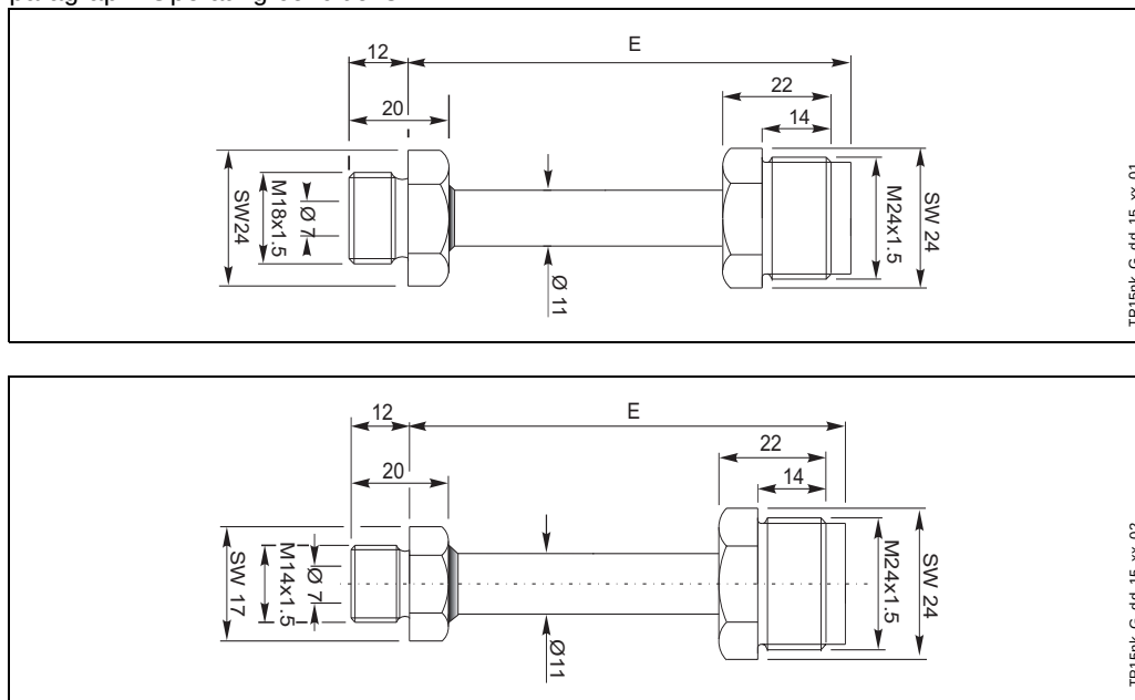
Fig. 8: Extension neck dimensions
