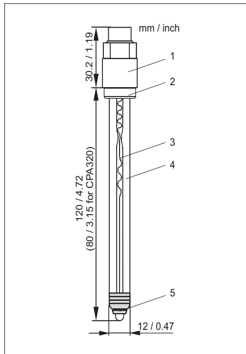
CPS13 with GSA plug-in head
