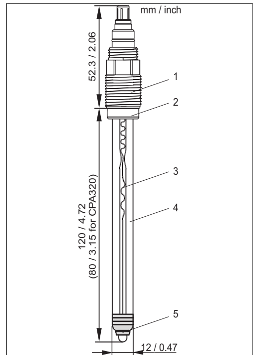
CPS13 with TOP68 plug-in head
