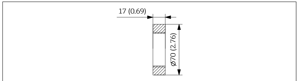
31 Dimensions weld-in adapter FAR52. Unit of measurement mm (in)
