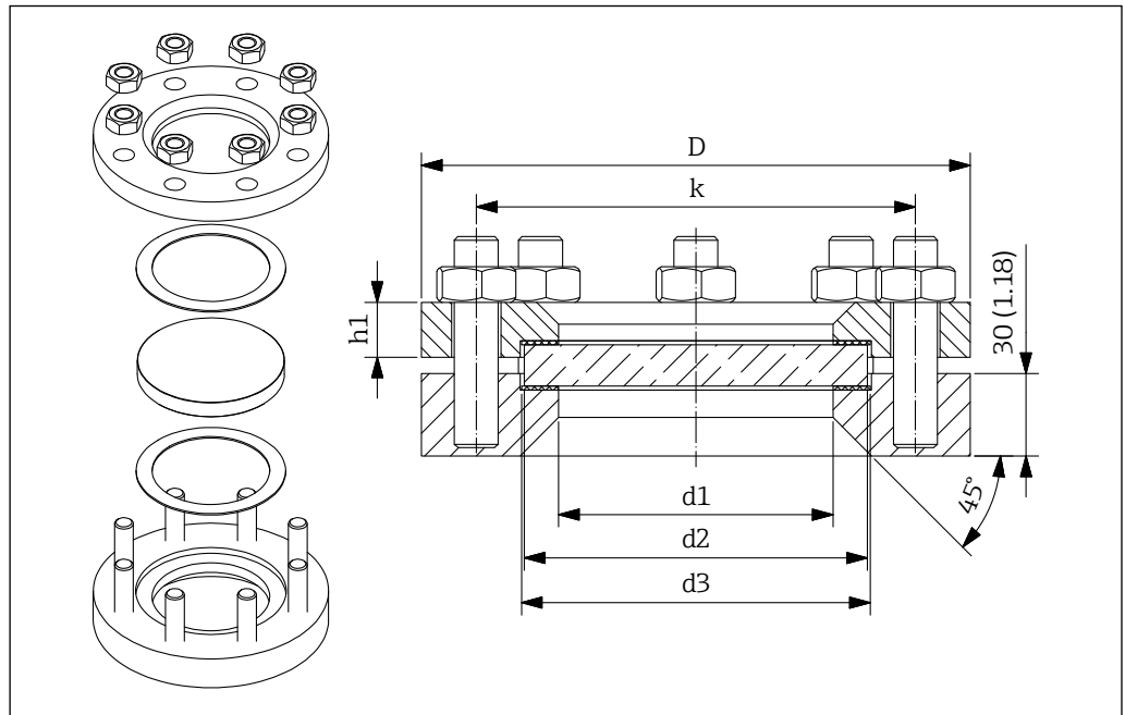
37 Dimensions sight glass fitting for processes up to 10 bar (145 psi). Unit of measurement mm (in)
