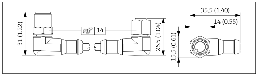
■ 27 Connecting cable with M12 right-angle plug and M12 right-angle socket. Unit of measurement mm (in) 0000000135
