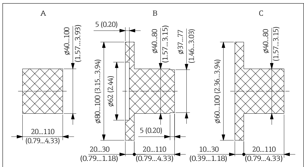
35 Dimensions plug FAR54. Unit of measurement mm (in)
