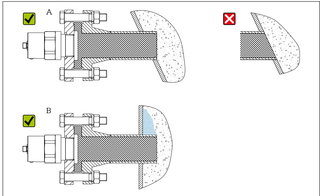
17 Mounting with risk of buildup
