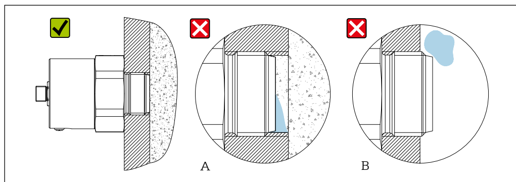
9 Direct mounting with threaded connection
