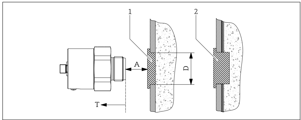
13 Mounting in front of microwave-impermeable process wall
