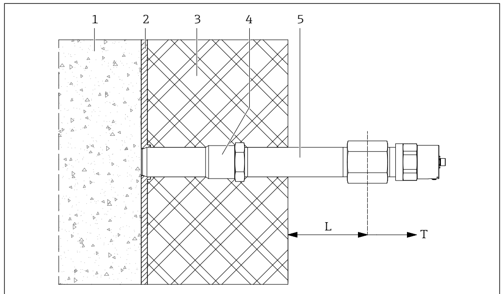
20 Mounting with high temperature adapter and extensions
