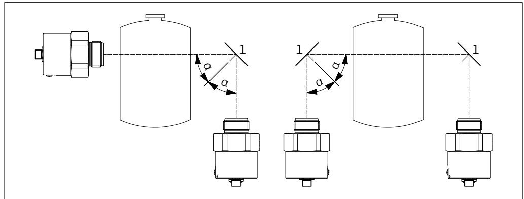
7 Reflector operation
