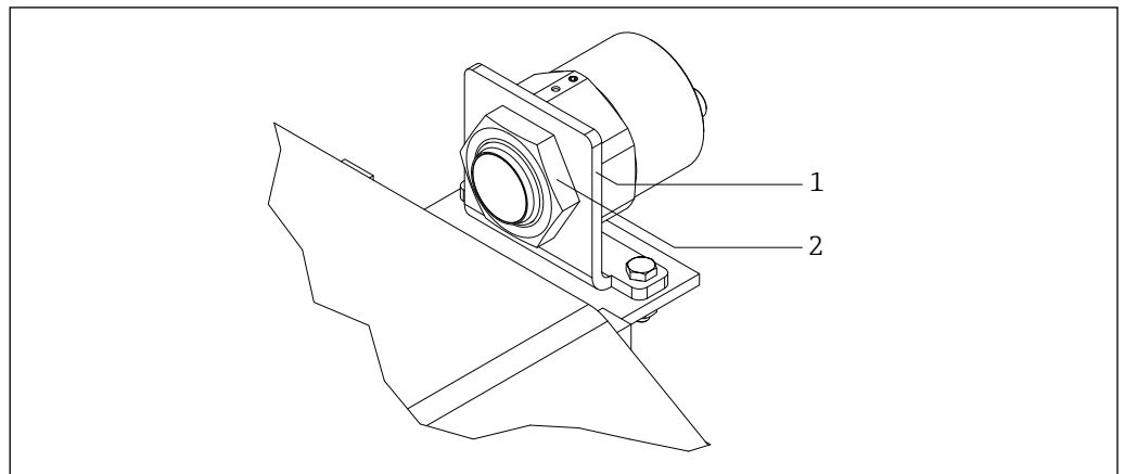
21 Mounting for open processes
