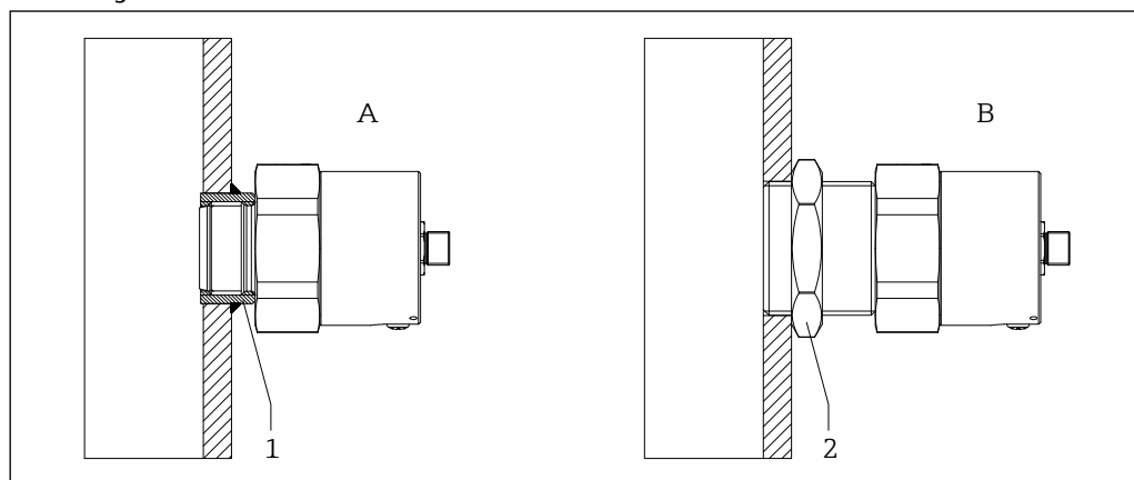
12 Mounting alternatives
