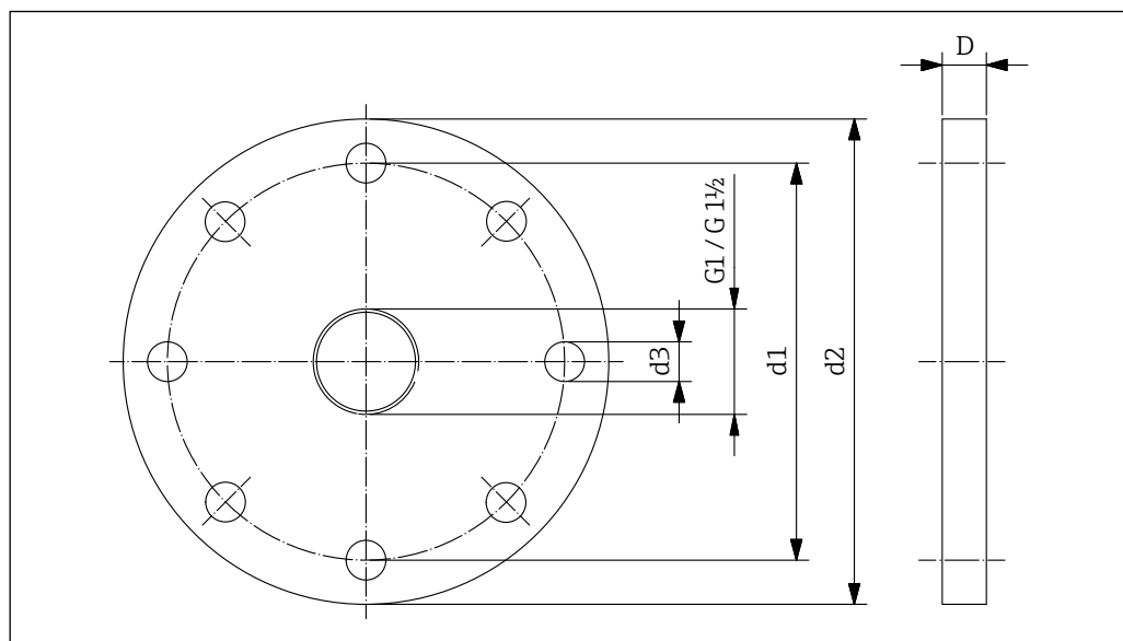
32 Dimensions mounting flange (Connection dimensions according to DIN EN 1092-1)
