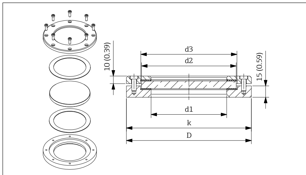
36 Dimensions sight glass fitting for unpressurized processes. Unit of measurement mm (in)
