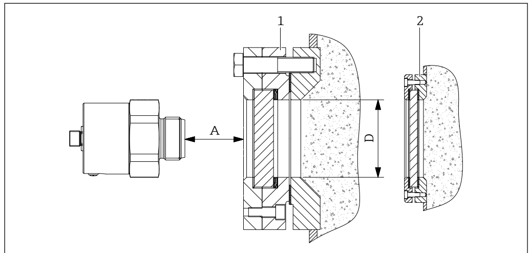
14 Mounting in front of microwave permeable sight glass fitting
