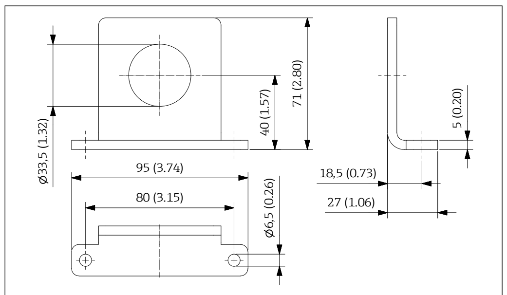
■ 29 Dimensions mounting bracket. Unit of measurement mm (in) 0000000037
