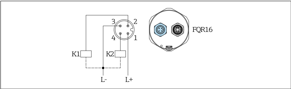
4 Electrical connection
