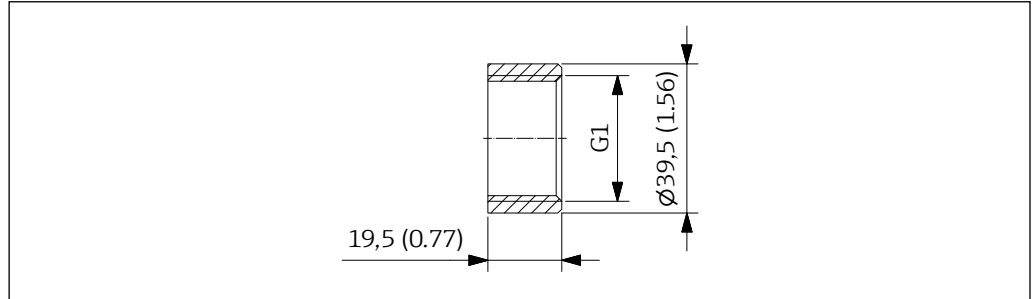
30 Dimensions welding sleeve. Unit of measurement mm (in)
