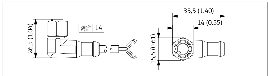
■ 26 Connection cable with M12 right-angle socket. Unit of measurement mm (in)
