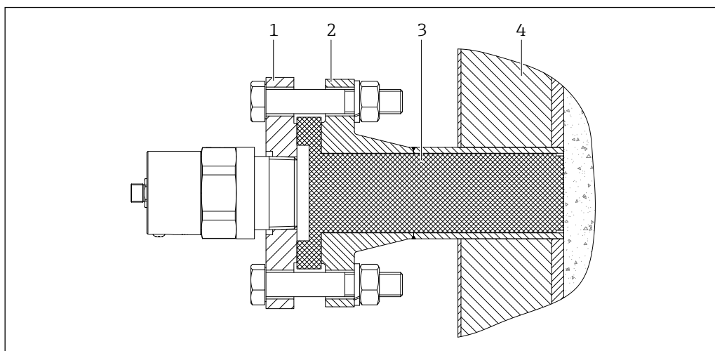
16 Mounting on process nozzle
