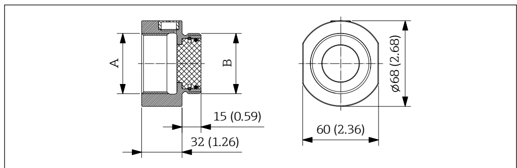
34 Dimensions high pressure adapter. Unit of measurement mm (in)
