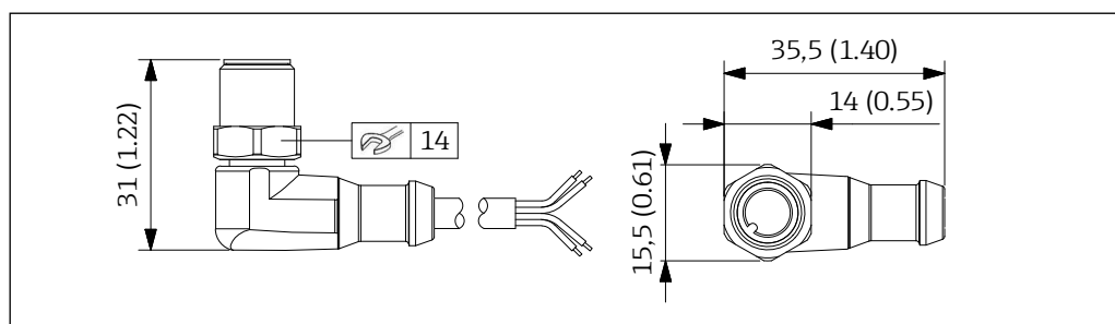
25 Connection cable with M12 right-angle plug. Unit of measurement mm (in)
