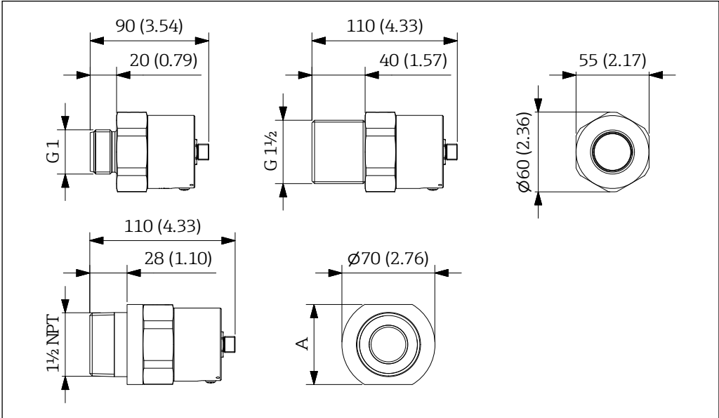
22 Dimensions. Unit of measurement mm (in)
