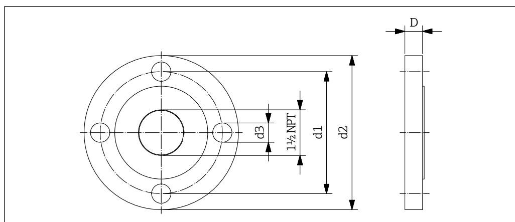
33 Dimensions mounting flange (Connection dimensions according to ANSI/ASME B16.5)
