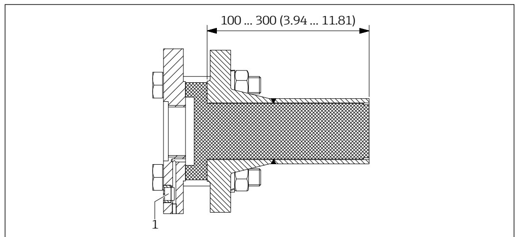
39 Dimensions weld-in nozzle. Unit of measurement mm (in)
