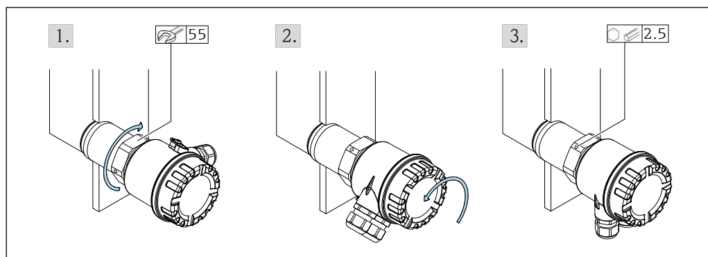
15 Mounting with connection thread
