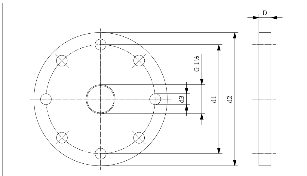
36 Dimensions mounting flange (Connection dimensions according to DIN EN 1092-1)
