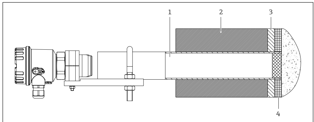
26 Mounting with spacer tube (wave guide)
