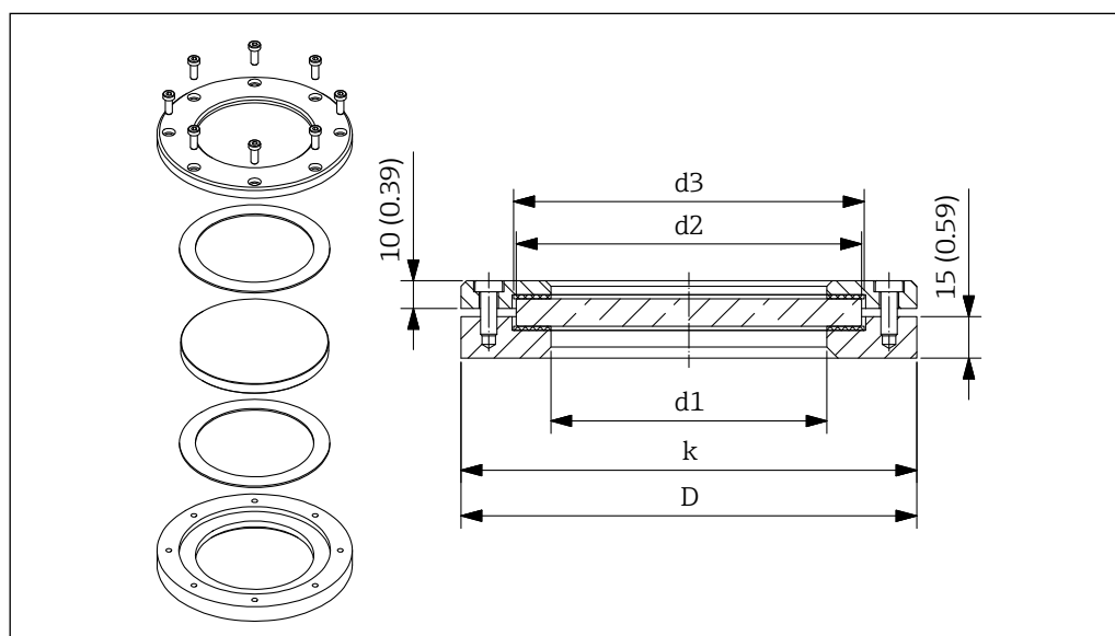
40 Dimensions sight glass fitting for unpressurized processes. Unit of measurement mm (in)
