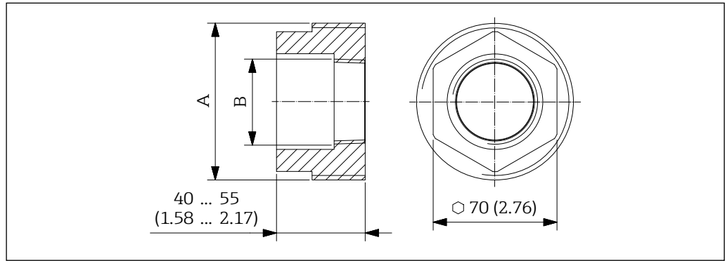
34 Dimensions FAR52-B. Unit of measurement mm (in)
