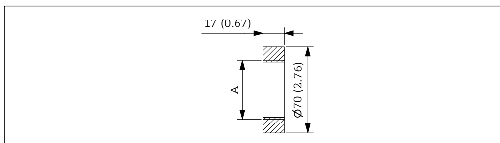
33 Dimensions FAR52-A. Unit of measurement mm (in)
