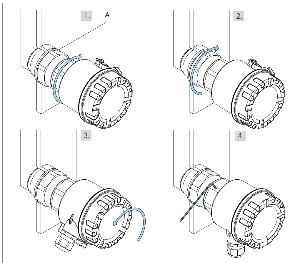
10 Installation with connection thread
