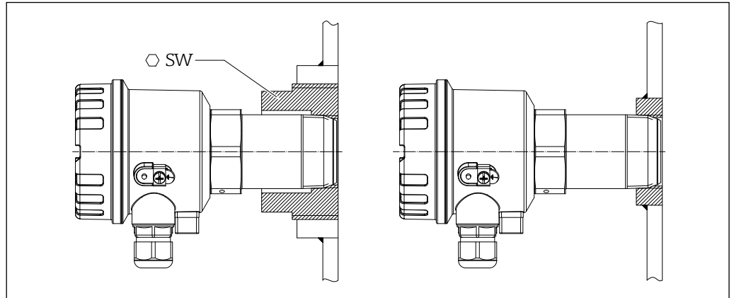
9 FAR52 weld-in or screw-in adapter
