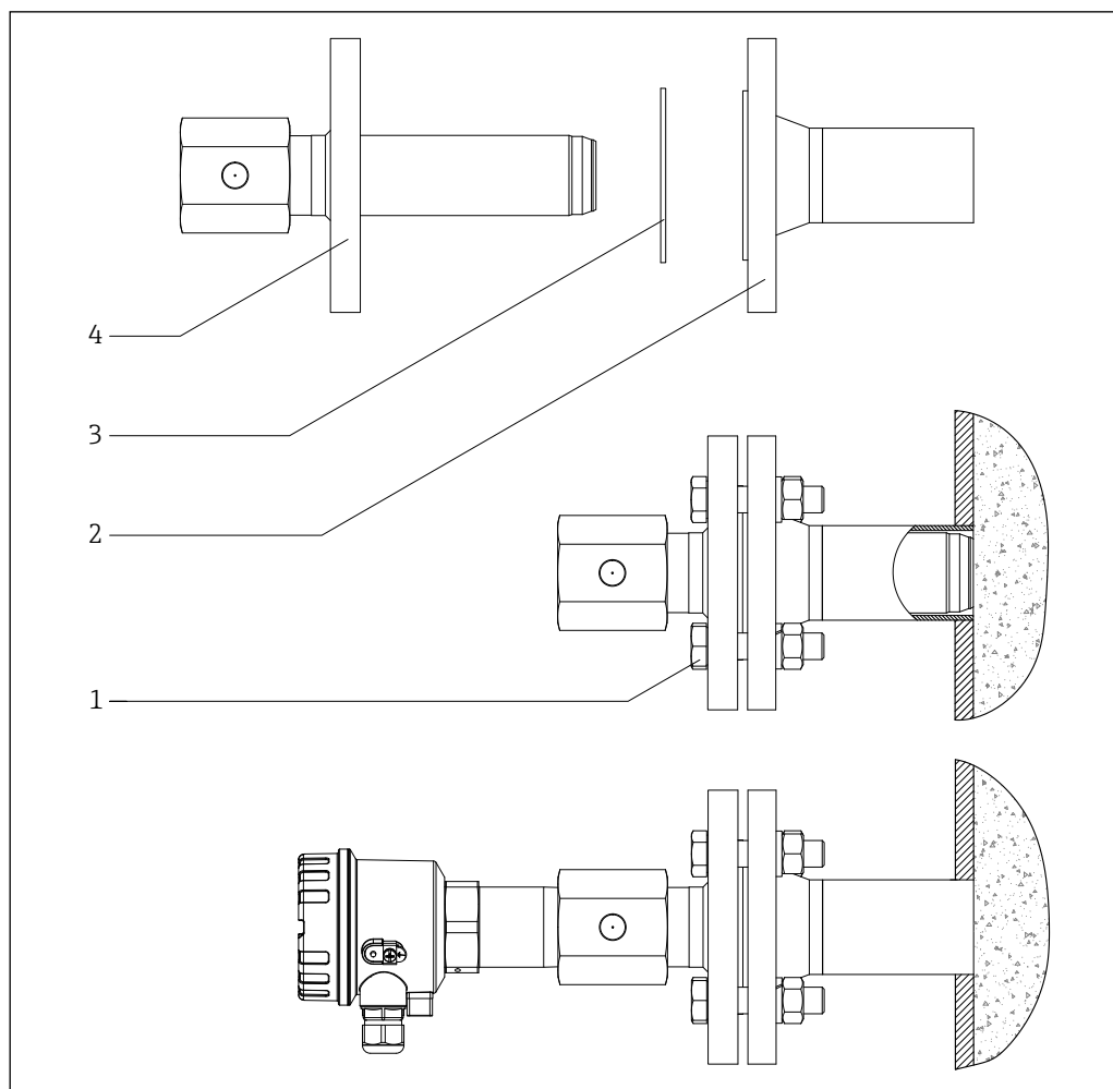
16 Mounting with FAR51 insertion adapter
