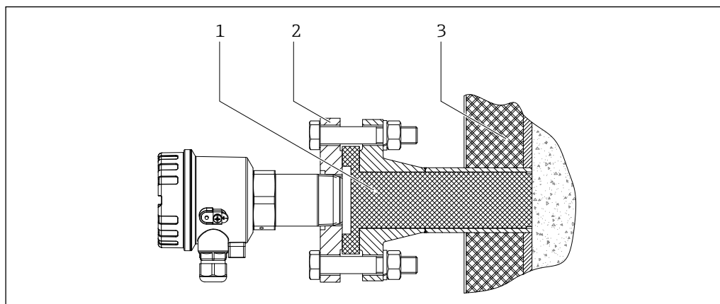
■ 14 Mounting on available process nozzles
