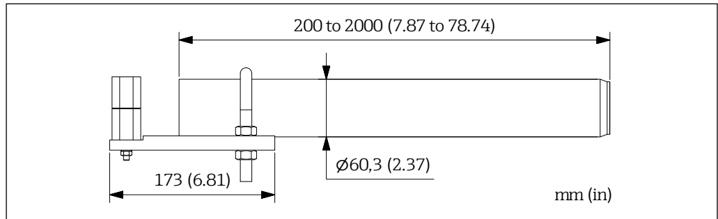
35 Dimensions of spacer tube (wave guide)
