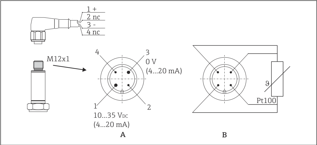
2 Pin assignment, device plug A Version with transmitter, M12 plug, 4-pin B Version without transmitter, Pt100, 4-wire connection
