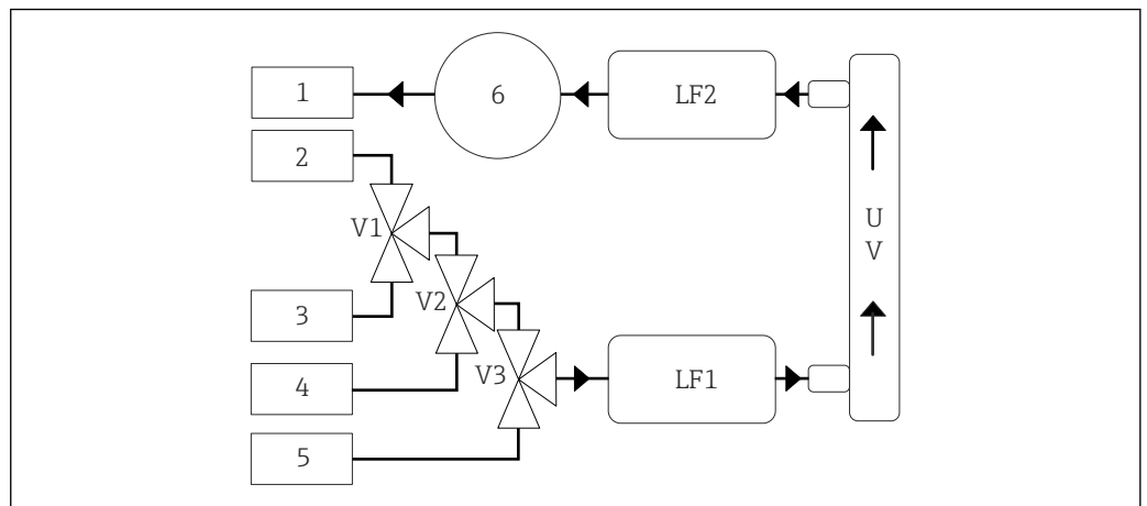
1 Process diagram
