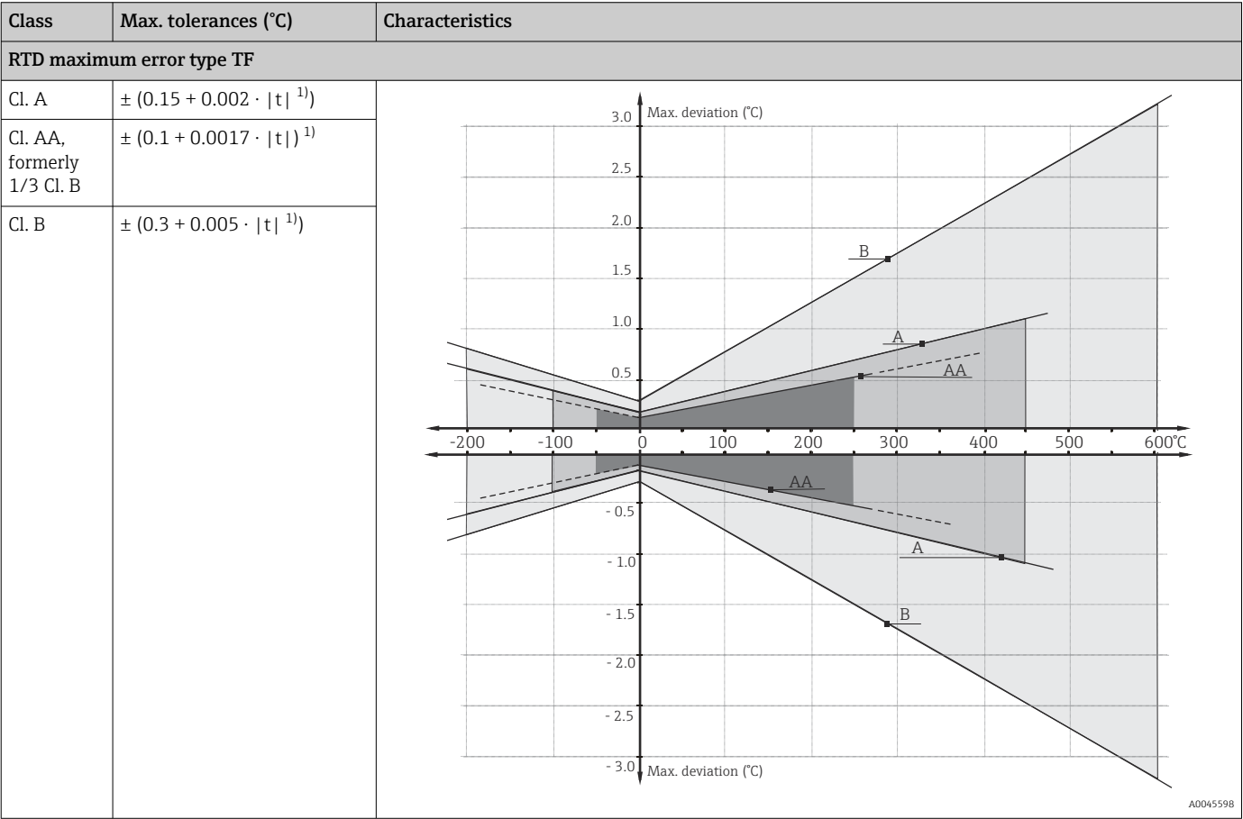
RTD resistance thermometer corresponding to IEC 60751
