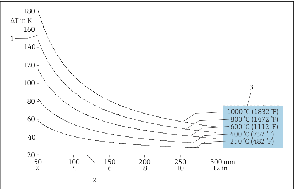
8 Heating of the terminal head as a function of the process temperature. Temperature in terminal head = ambient temperature 20 °C (68 °F) + \Delta T
