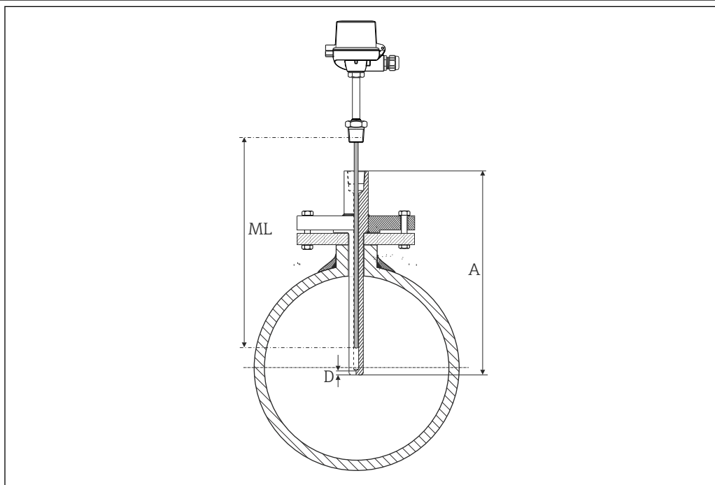
7 Thermometer installation
