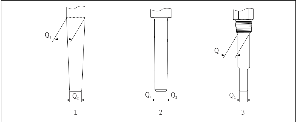
2 Thermowell shapes
