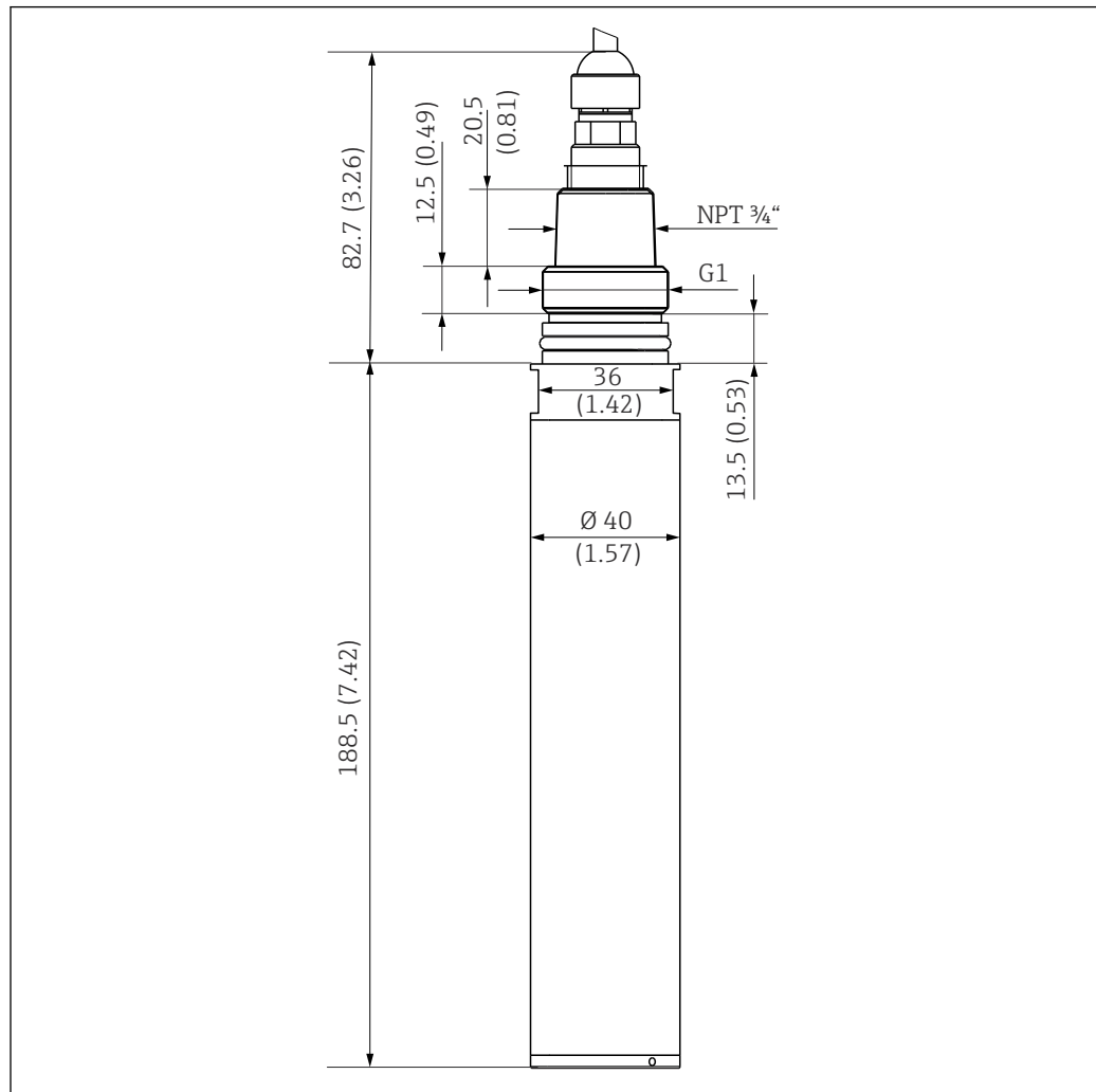
20 Dimensions. Engineering unit: mm (in)
