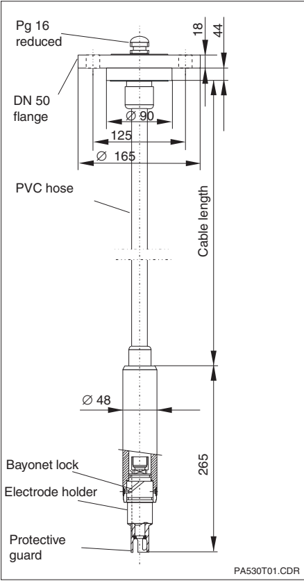
left: CPA 530 with flange right: CPA 530 with mounting bracket
