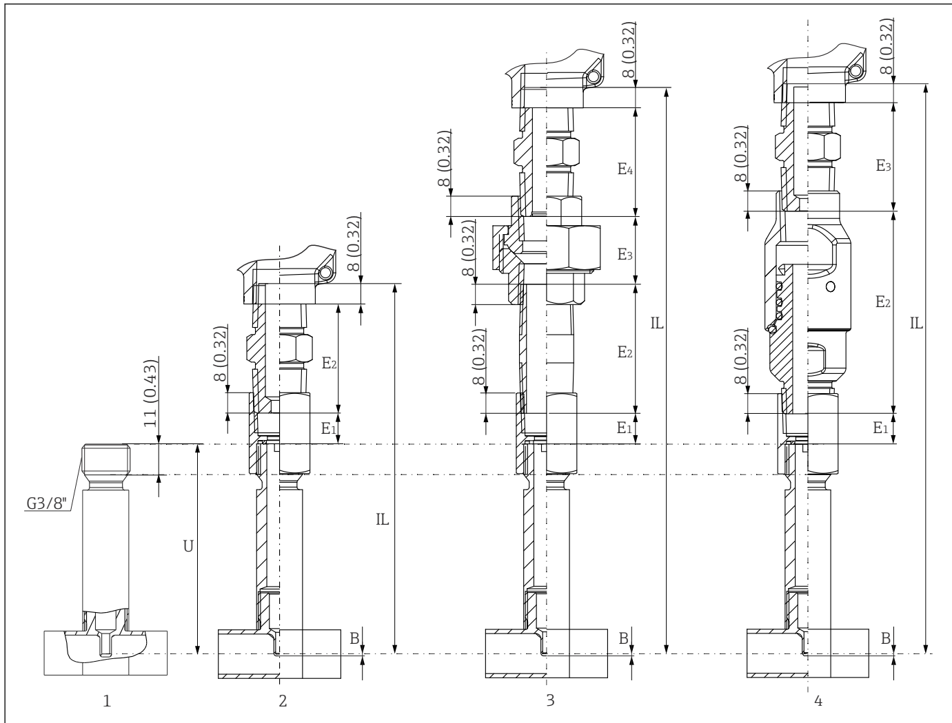
13 Tee thermowell as per DIN 11865 or ASME BPE
