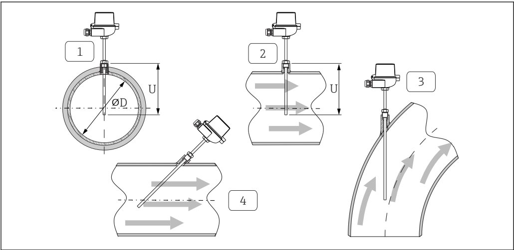
12 Installation examples
