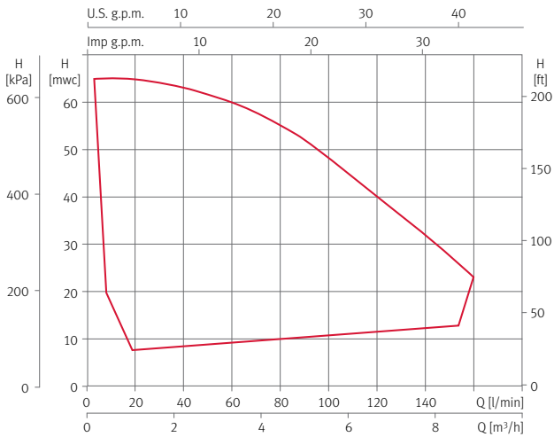
Performance area Aspri ESDM B at 2900 rpm
