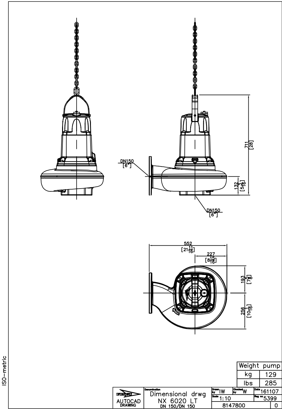
Figure 3: DN 150 (LT)
