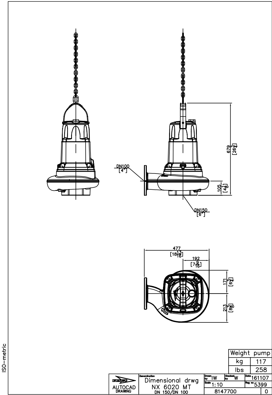
Figure 4: DN 100 (MT)
