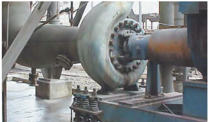
Installation for a difficult high-temperature service. Spring-mounted baseplate provided to compensate for thermal expansion.
