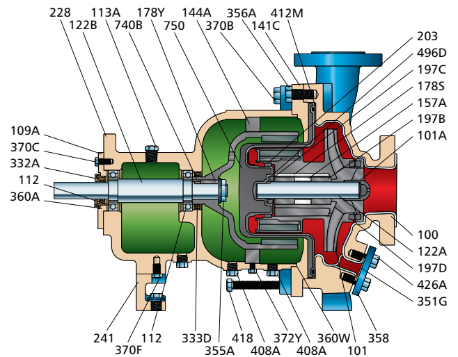
3298 M Frame-Mounted
