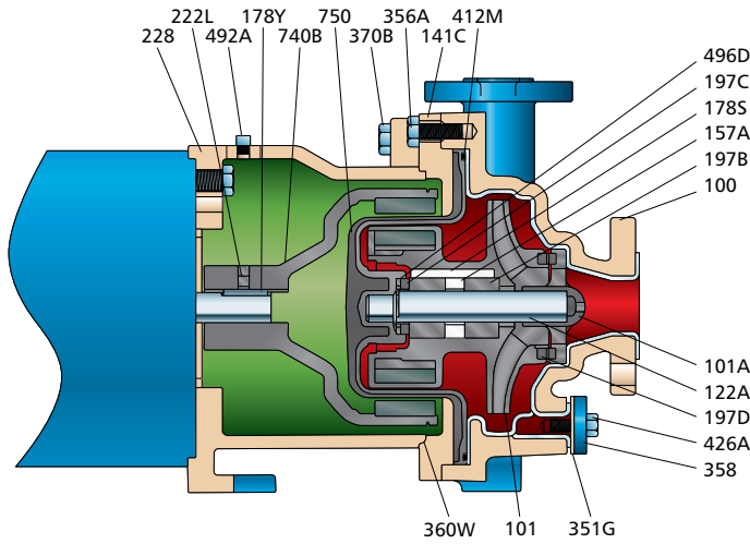
3298 S Close-Coupled
