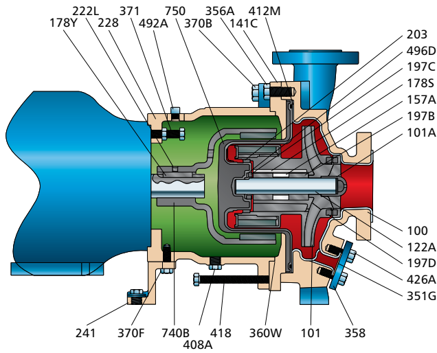
3298 M Close-Coupled
