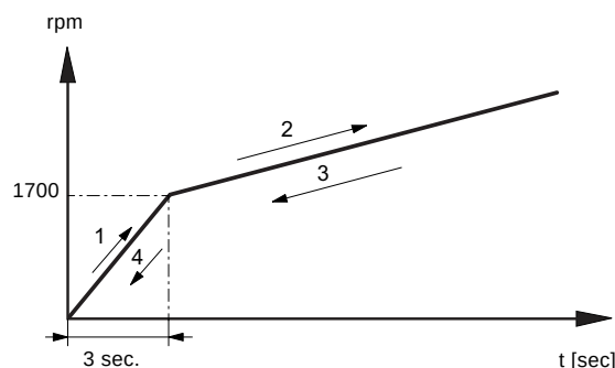
Fig. 12 Ramp times
