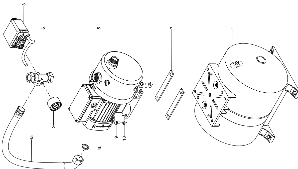
JP Booster with pressure tank
