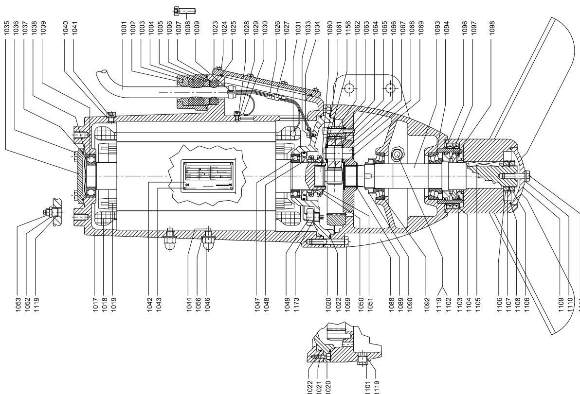
AMG.55.xxx.Ex - AMG.110.xxx.Ex (50 Hz only)
