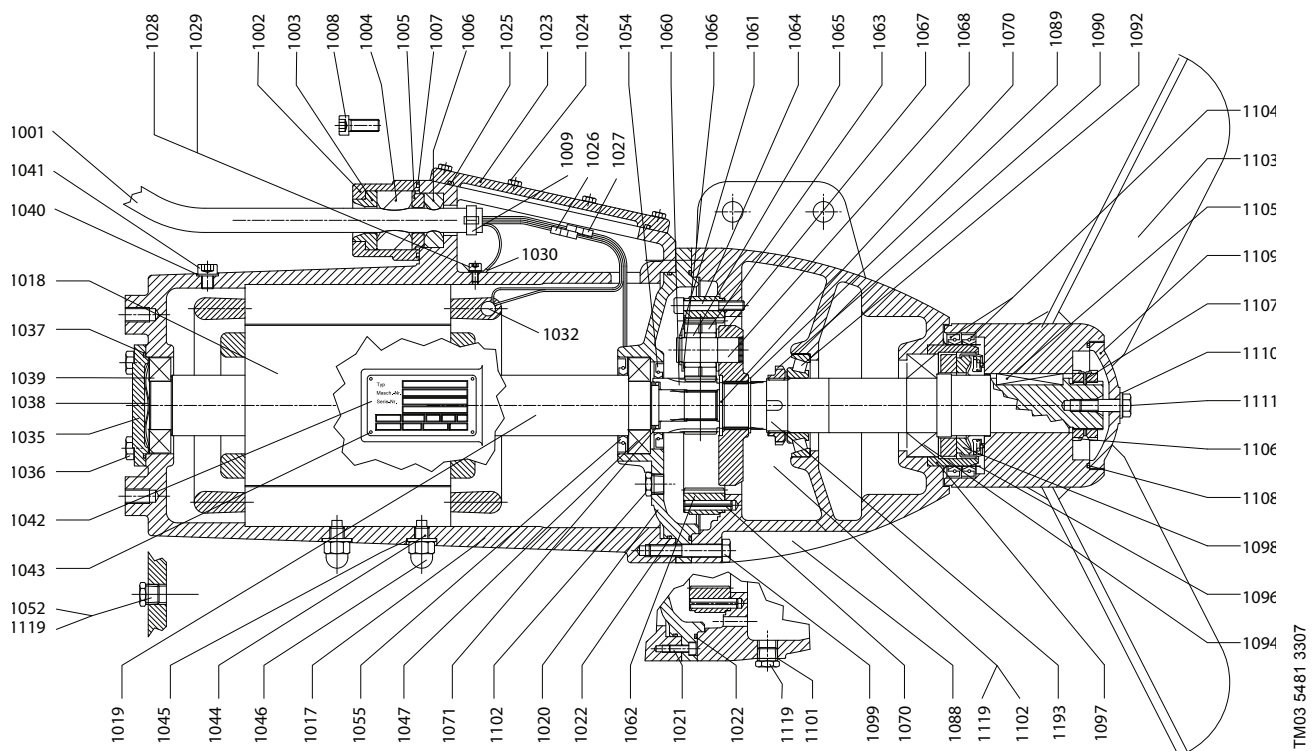
AMG.55.xxx.Ex - AMG.110.xxx.Ex (50 Hz only)
