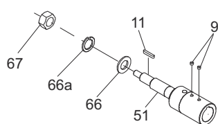
Stub shaft
