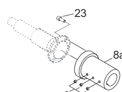
Motor bush
