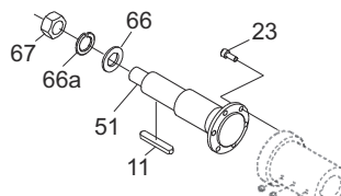
Pump shaft
