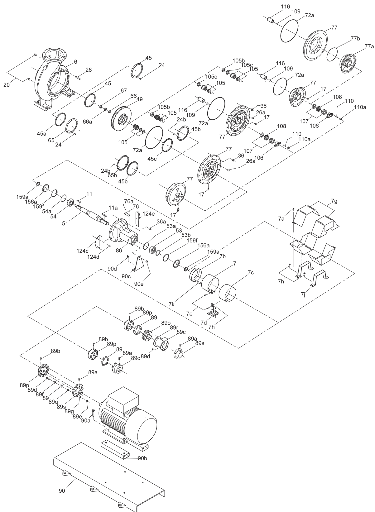
Fig. 6 Exploded view
