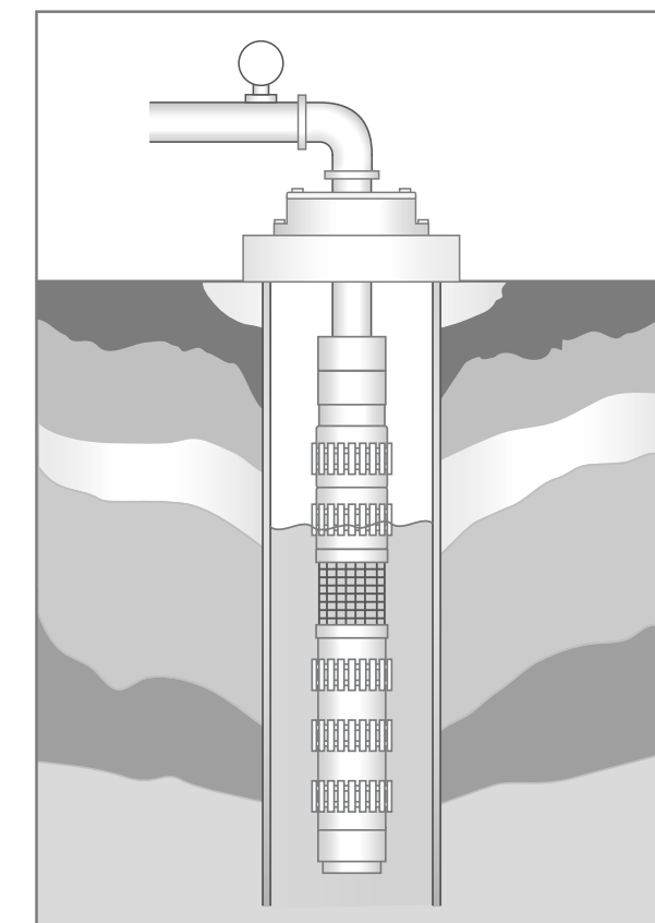
Fig. 67 Submersible pump set with sacrificial zinc anodes.
