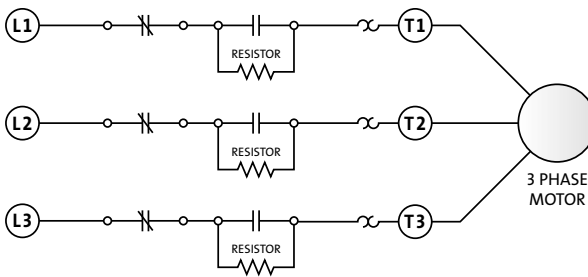
Fig. 36. Typical electrical diagram for a primary resistor reduced voltage starter
