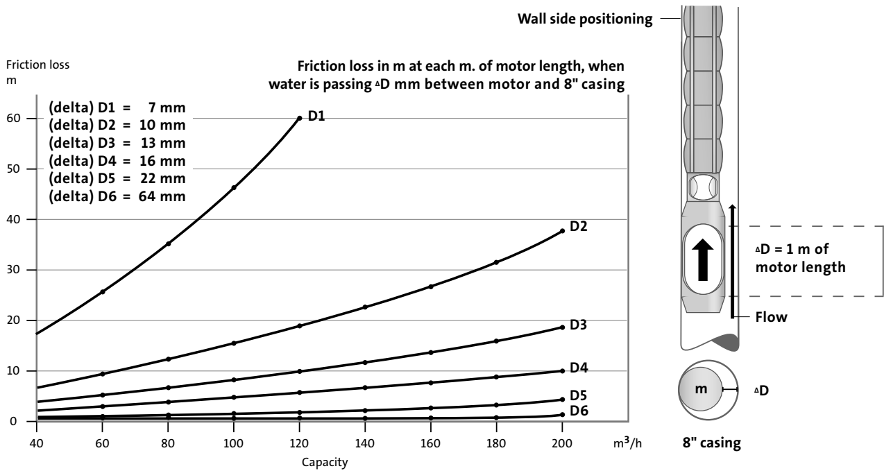
Fig. 53 Friction loss, 8"
