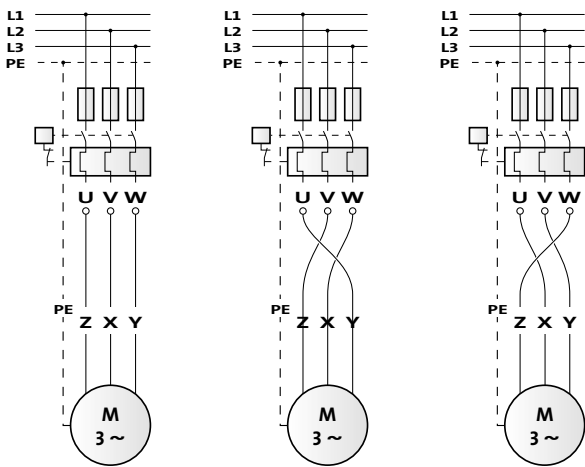
Fig. 47 Optimal connection
