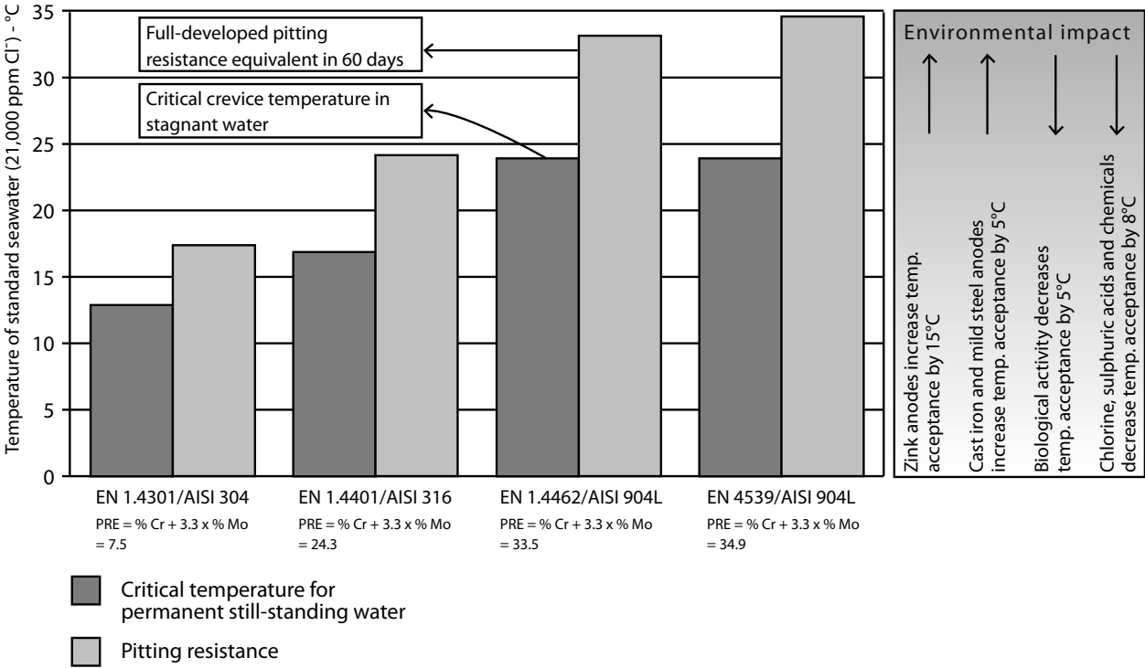
Fig. 16 Corrosion resistance
