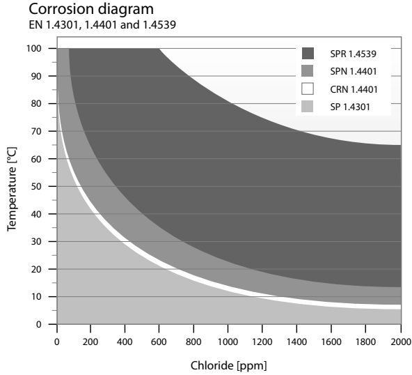
Fig. 17 Corrosion diagram
