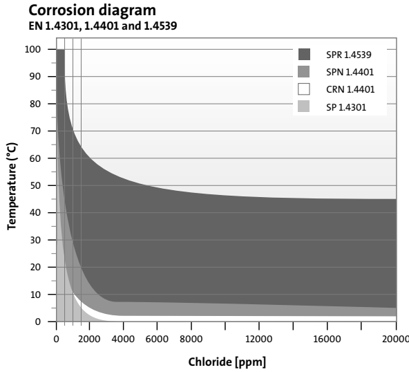
Fig. 18 Corrosion diagram
