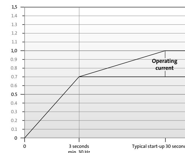
Fig. 40 Current flow by frequency converter starting
