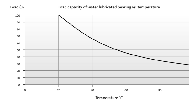
Fig. 45 Diagram: Journal bearings load capacity as function of motor liquid temperature.
