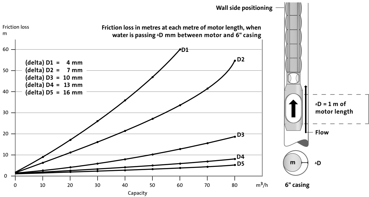
Fig. 52 Friction loss, 6"
