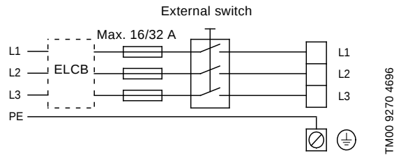
Fig. 91 Wiring diagram, three-phase MGE motors, 0.75 - 7.5 kW
