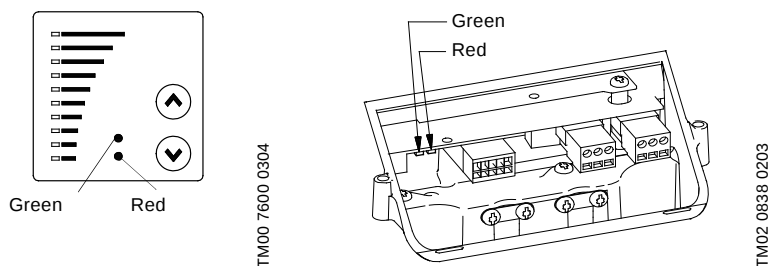
Fig. 84 Position of indicator lights on single-phase pumps
