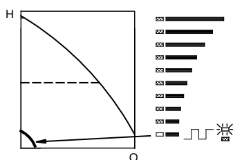
Fig. 70 Min. curve duty
