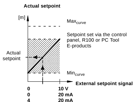
Fig. 40 Relation between the actual setpoint and the external setpoint signal in control mode "Uncontrolled"
