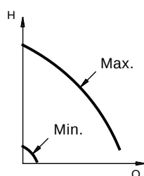
Fig. 63 Min. and max. curves
