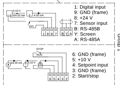
Fig. 88 Connection terminals
