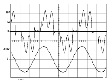
Fig. 114 Mains current and voltage for a) a standard asynchronous motor and b) a three-phase MGE motor
