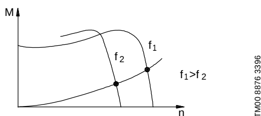
Fig. 110 Displacement of motor torque characteristic
