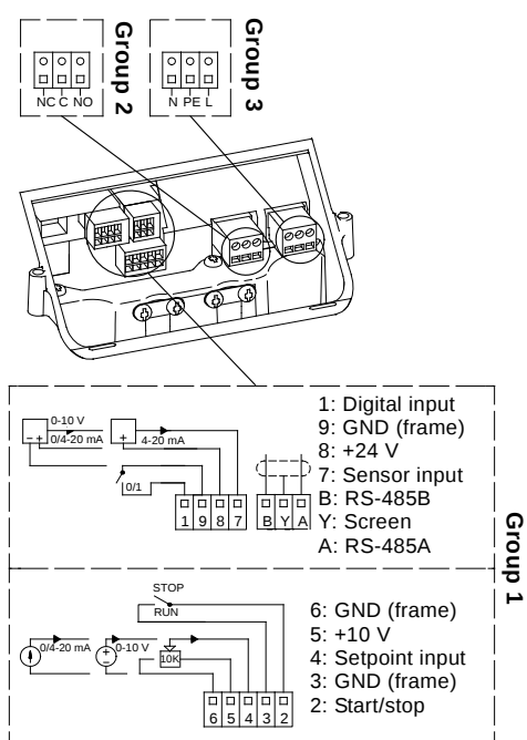
Fig. 56 Connection terminals, TPE, NKE and NBE
