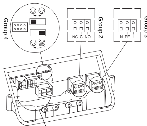
Fig. 88 Connection terminals
