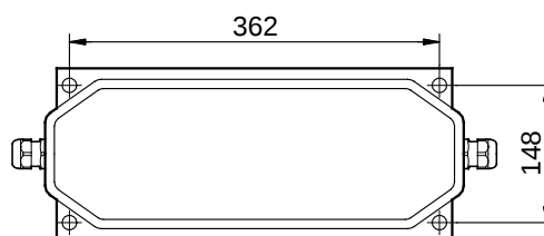
Fig. 143 Dimensional sketch
