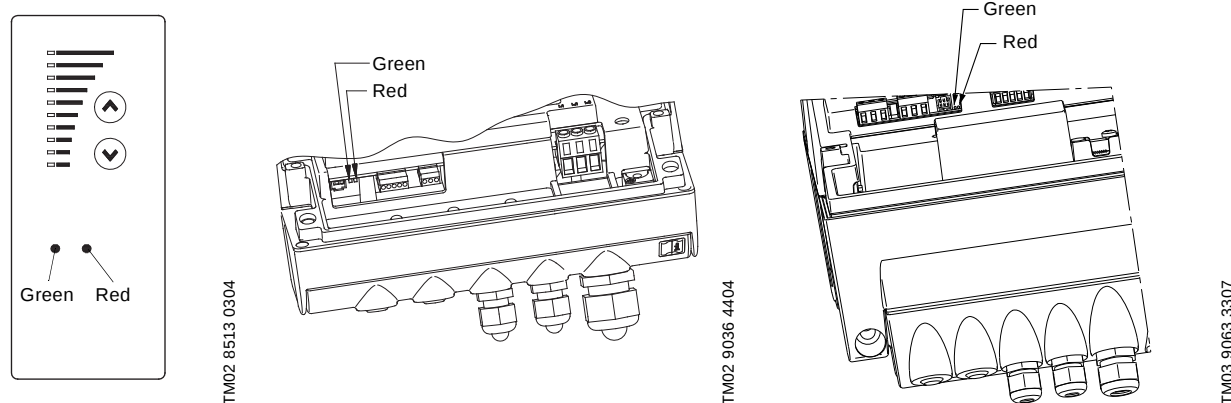
Fig. 85 Position of indicator lights on three-phase pumps
