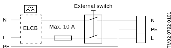
Fig. 87 Wiring diagram, single-phase MGE motors
