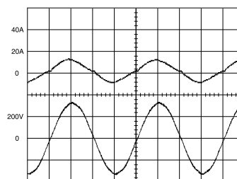
Fig. 115 Mains voltage and current for a 1.1 kW MGE motor with PFC circuit
