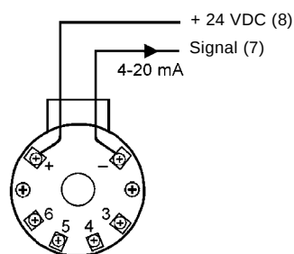
Fig. 138 Connection of sensor
