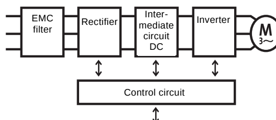
Fig. 111 The main blocks of a frequency converter
