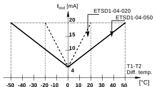
Fig. 139 Sensor characteristic
