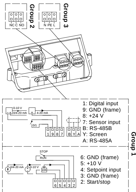
Fig. 37 Connection terminals
