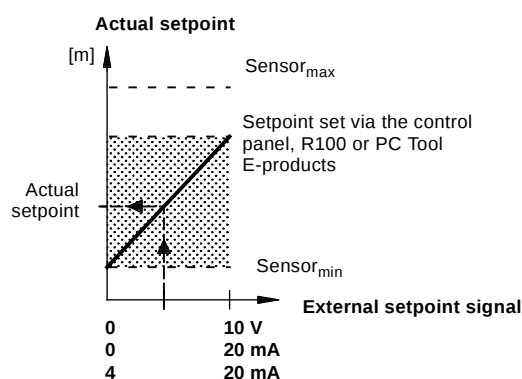
Fig. 39 Relation between the actual setpoint and the external setpoint signal in control mode "Controlled"
