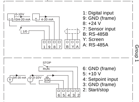
Fig. 92 Connection terminals
