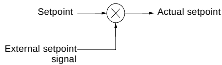
Fig. 57 Actual setpoint as a product (multiplied value) of setpoint and external setpoint signal
