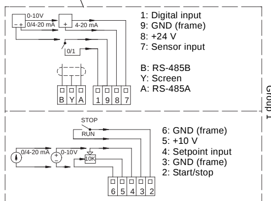
Fig. 89 Connection terminals, TPED Series 2000
