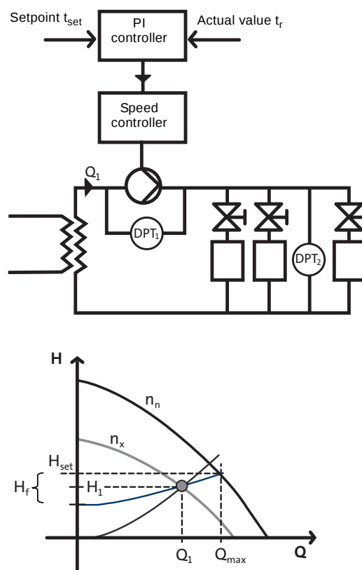
Fig. 16 Flow-compensated differential-pressure control
