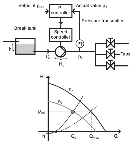
Fig. 13 Constant-pressure control
