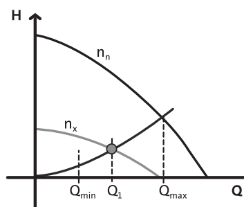
Fig. 14 Constant-temperature control
