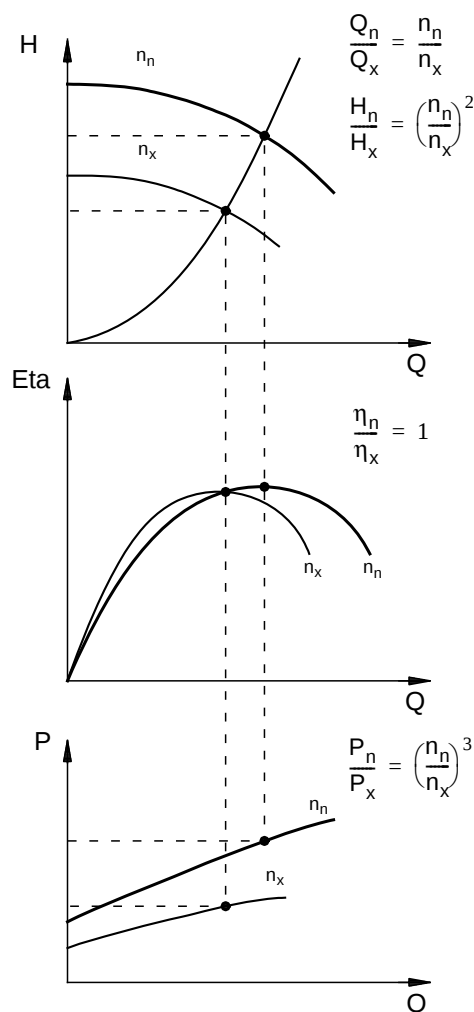
Fig. 6 Affinity equations
