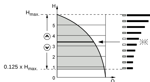
Fig. 68 Pump in control mode "Constant pressure"
