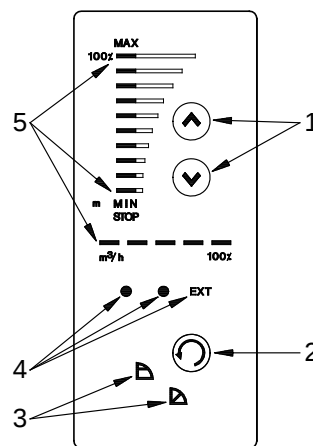
Fig. 71 Control panel, three-phase pumps, 0.55 - 22 kW
