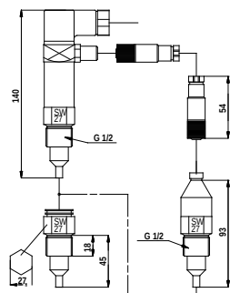
Fig. 140 Dimensional sketch
