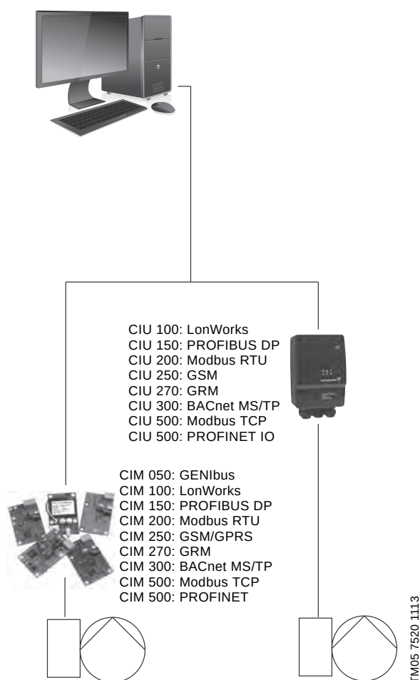
Fig. 85 Structure of a central building management system
