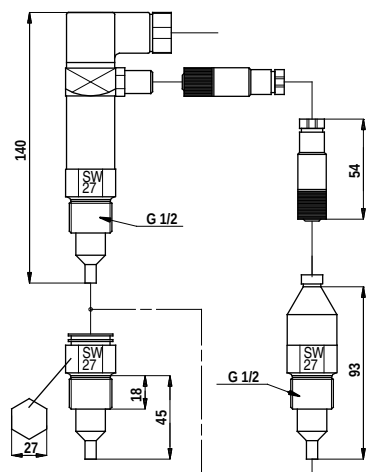
Fig. 116 Dimensional sketch
