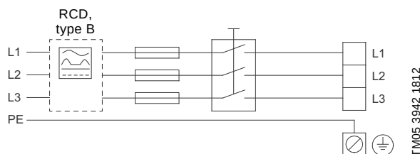
Fig. 105 Example of a mains-connected motor with main switch, backup fuse and additional protection
