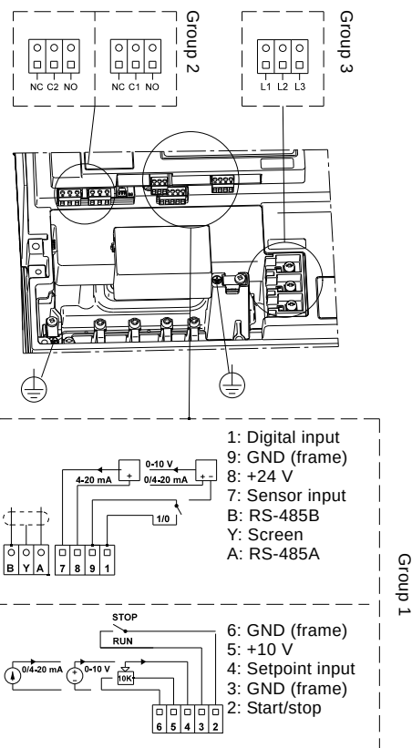
Fig. 108 Connection terminals
