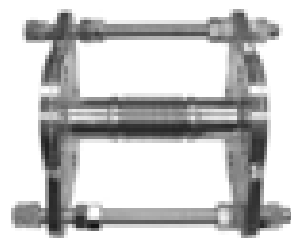
Fig. 101 Example of metal expansion joint
