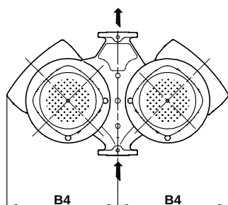
Fig. 103 Terminal box positions of TPED pumps
