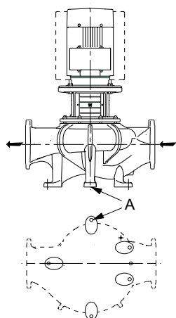
Fig. 111 Principal sketch of a Series 300 pump designed with mounting feet (A)
