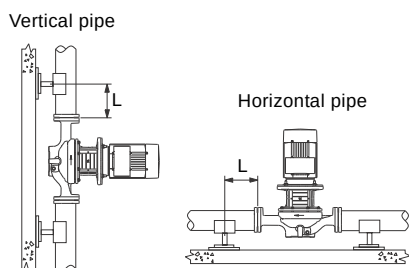
Fig. 92 Pump suspended directly in the pipes
