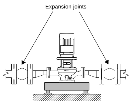
Fig. 99 TP pump installed with larger expansion joints
