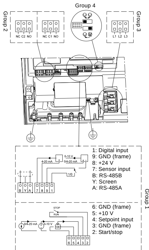
Fig. 109 Connection terminals, TPED Series 2000
