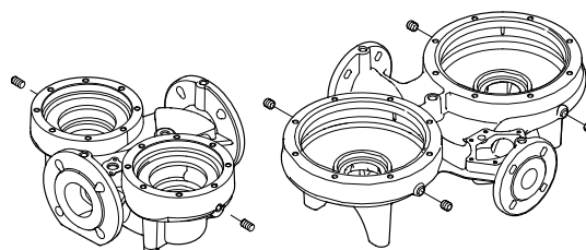
Fig. 94 Tappings for mounting of automatic vents in TP Series 200, TPE2 D, TPE3 D and TP Series 300
