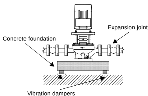
Fig. 97 Foundation of TP pump
