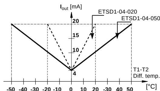
Fig. 115 Sensor characteristics
