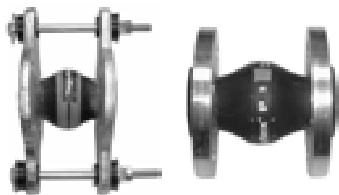
Fig. 100 Examples of rubber bellows expansion joints
