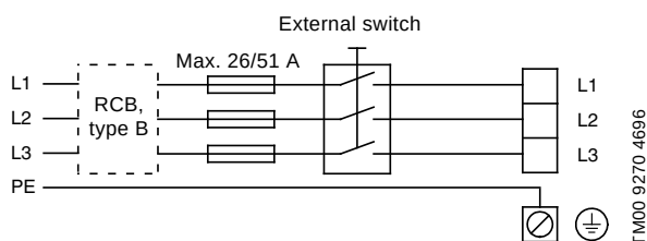
Fig. 107 Wiring diagram, three-phase MGE motors, 11-22 kW
