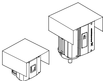
Fig. 96 Motors with condensation cover
