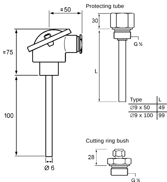
Fig. 114 Dimensional sketch
