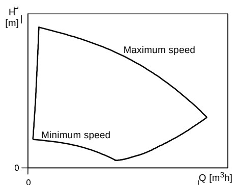
Fig. 23 Duty range of TPE2
