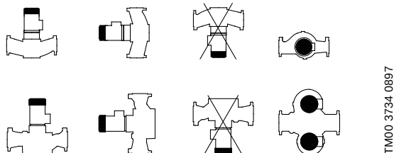
Fig. 90 Installation of motor sizes smaller than 11 kW
