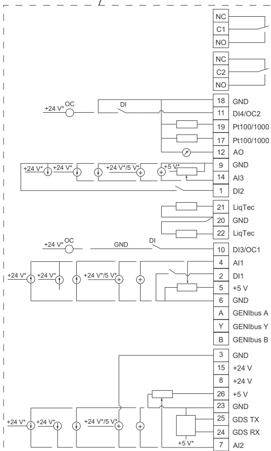
Fig. 106 Connection terminals, FM 300, option
