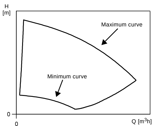
Fig. 86 Minimum and maximum performance curves
