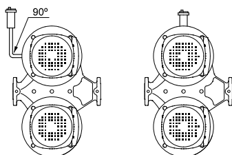
Fig. 93 Twin-head pumps with automatic vent
