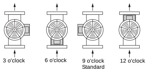
Fig. 102 Possible terminal box positions
