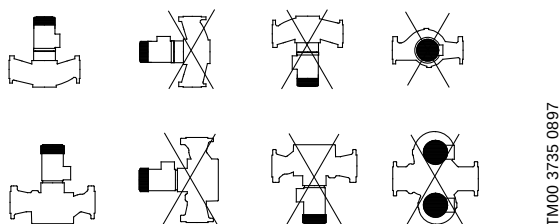
Fig. 91 Installation of motor sizes of 11 kW and up
