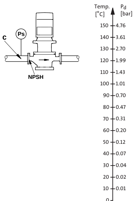
Fig. 123 Minimum inlet pressure
