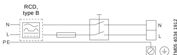
Fig. 104 Example of a mains-connected motor with main switch, backup fuse and additional protection
