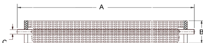
4040 Style with ATDs Core tube extension = 1.05" (26.7 mm)
