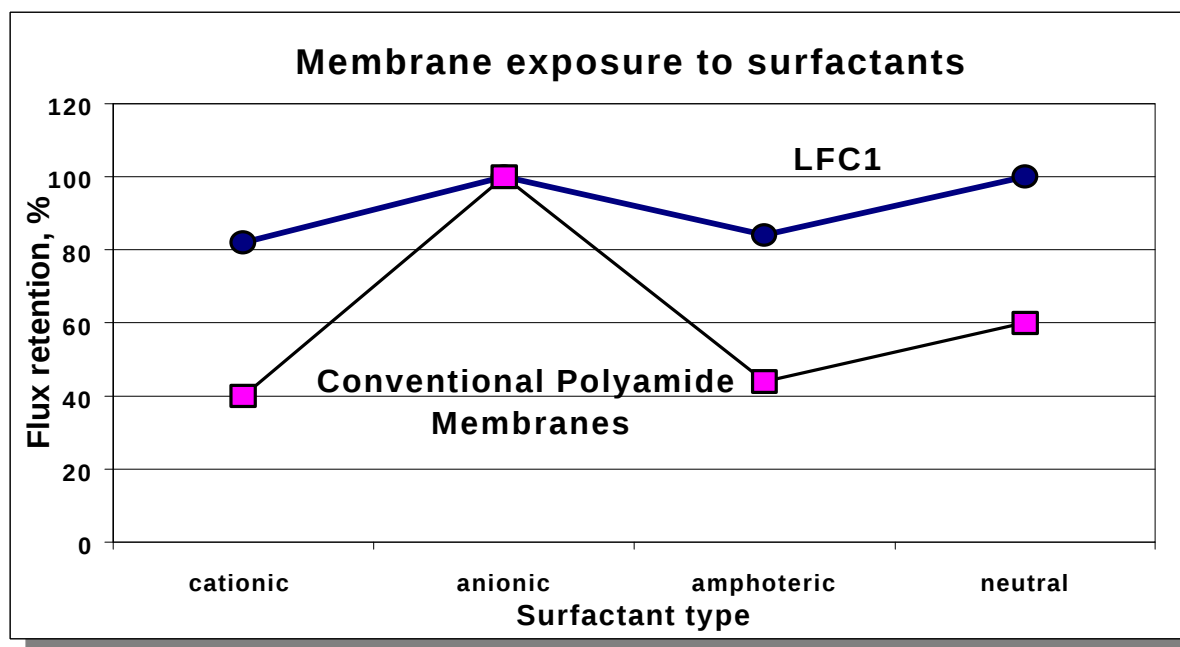
Graph 2: Surfactant effects on LFC1 and conventional membranes.
