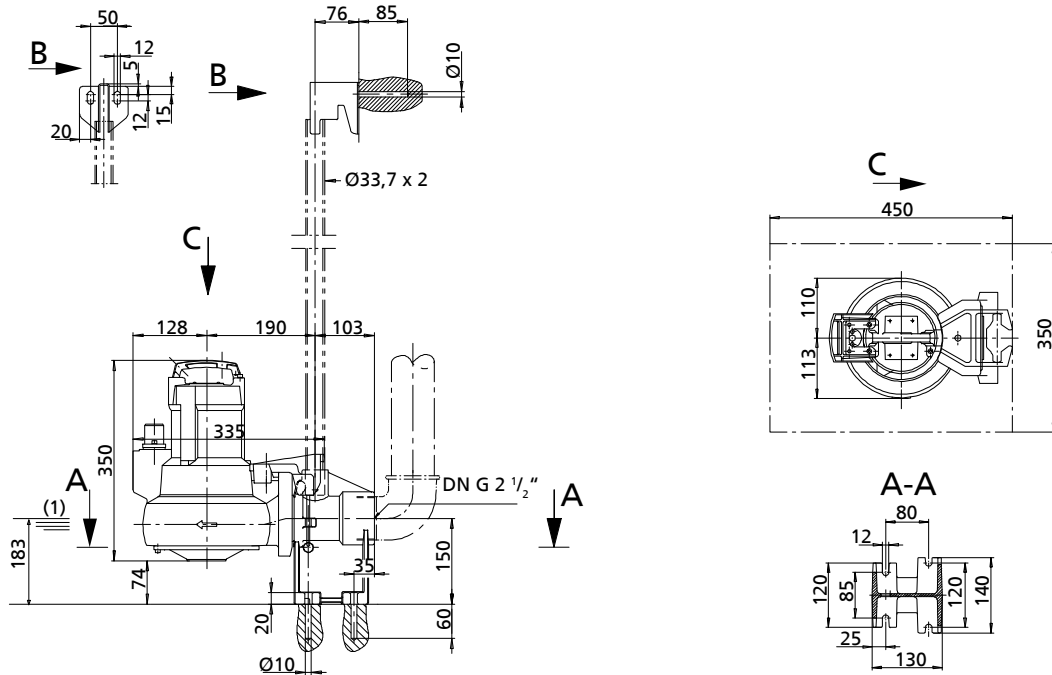
Ama-Porter 6 __, F impeller, stationary wet-installed model with single guide rail, straight pump foot G 2 1/2"
