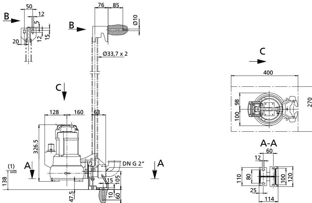
Ama-Porter S 545, S impeller, stationary wet-installed model with single guide rail, straight pump foot G 2"
