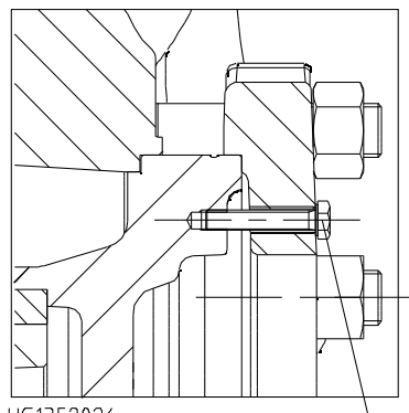
Model with clamped casing cover
