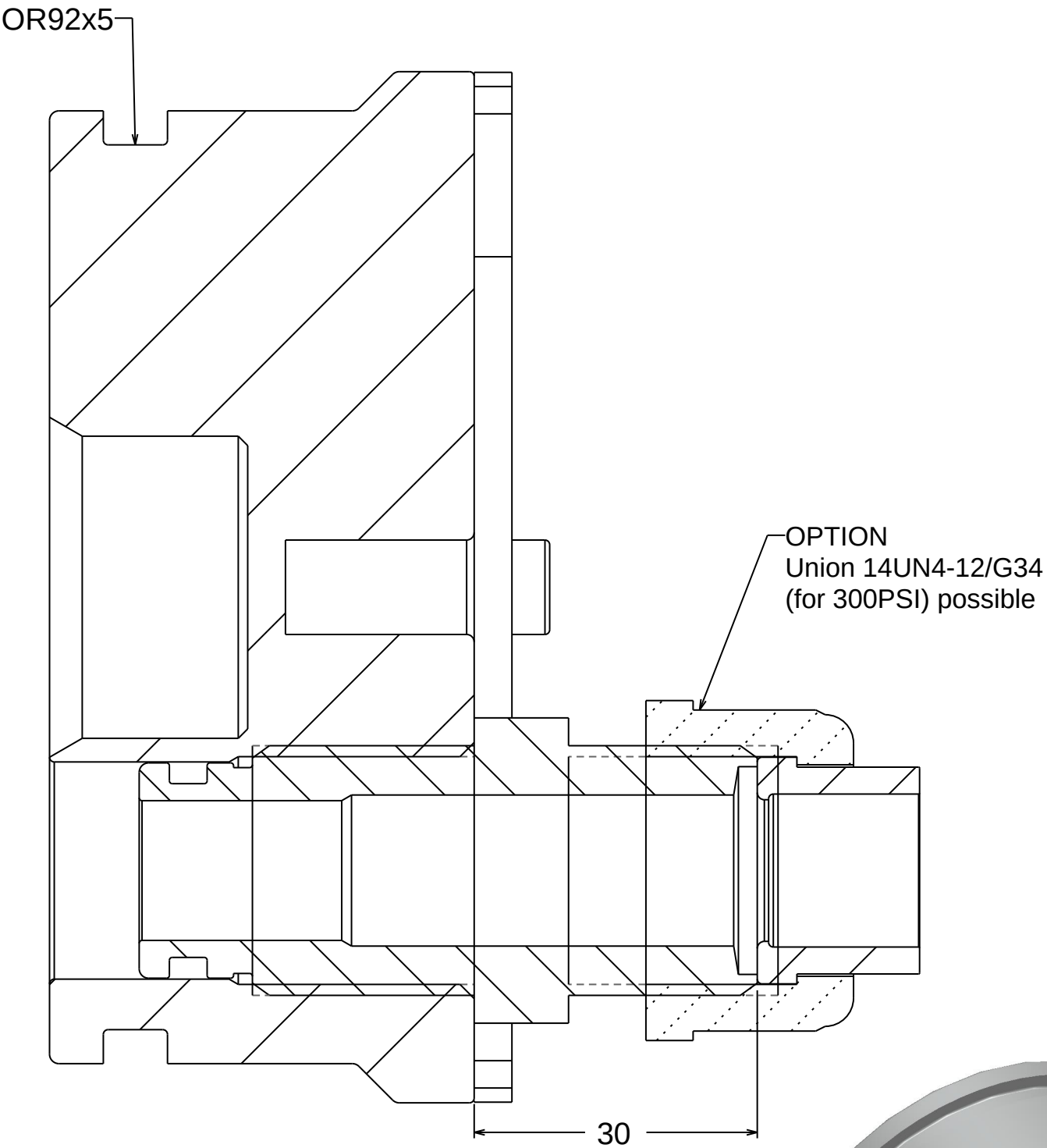
SECTION Y-Y
