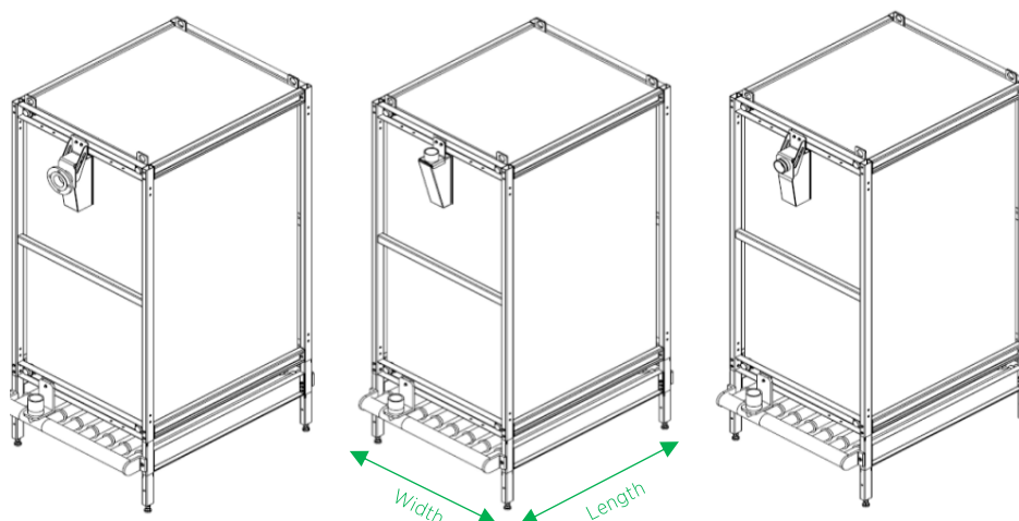
Left BIO-CEL L+ 480 FLANGE, Center BIO-CEL L+ 480 (Standard), Right BIO-CEL L+ 480 Vactaulic
