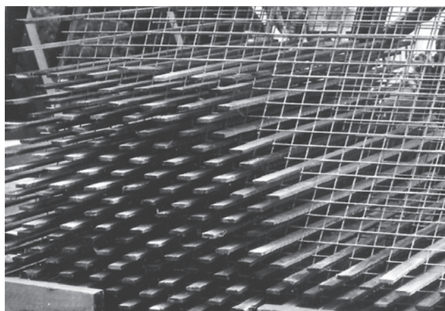
Wood Splash-type Fill
