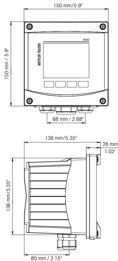
Dimension Drawing M400
