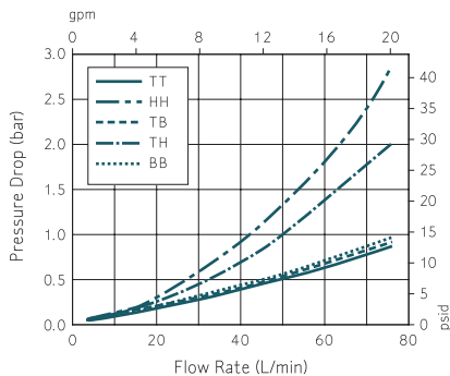
Opticap XLT 10 Capsule Filters with 0.2 \mu m Millipore Express SHF Membrane
