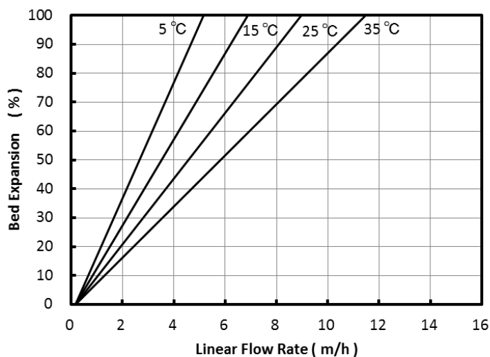
Fig. 2 Bed Expansion of NSA100
