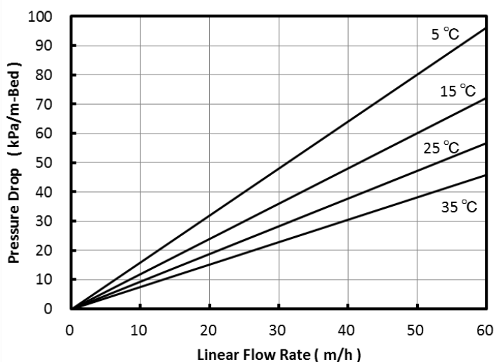
Fig. 1 Pressure Drop of NSA100
