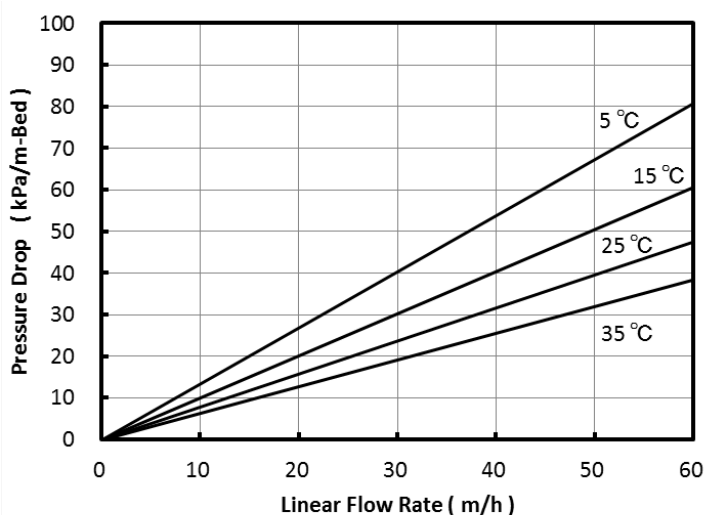
Fig. 1 Pressure Drop of PA312LTU
