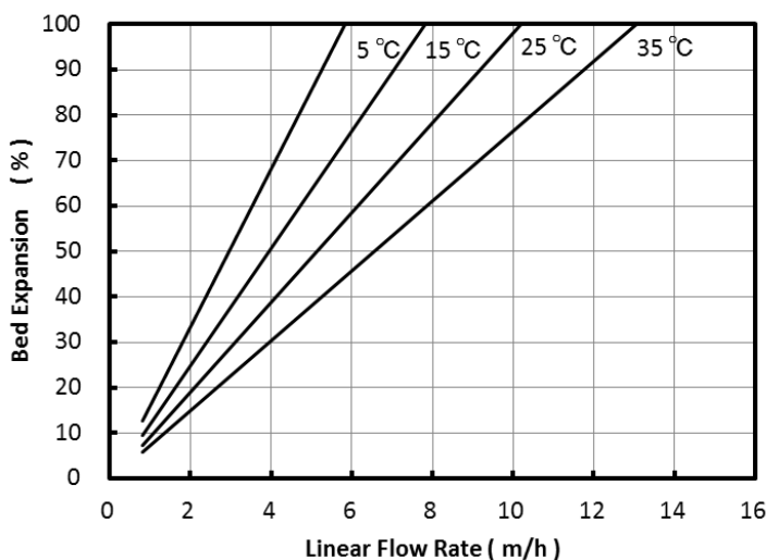
Fig. 2 Bed Expansion of PA312LTU
