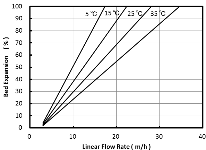
Fig. 2 Bed Expansion of PK212L
