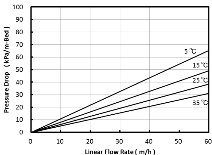
Fig. 1 Pressure Drop of PK212L
