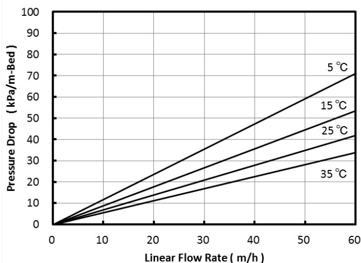
Fig. 1 Pressure Drop of PK220
