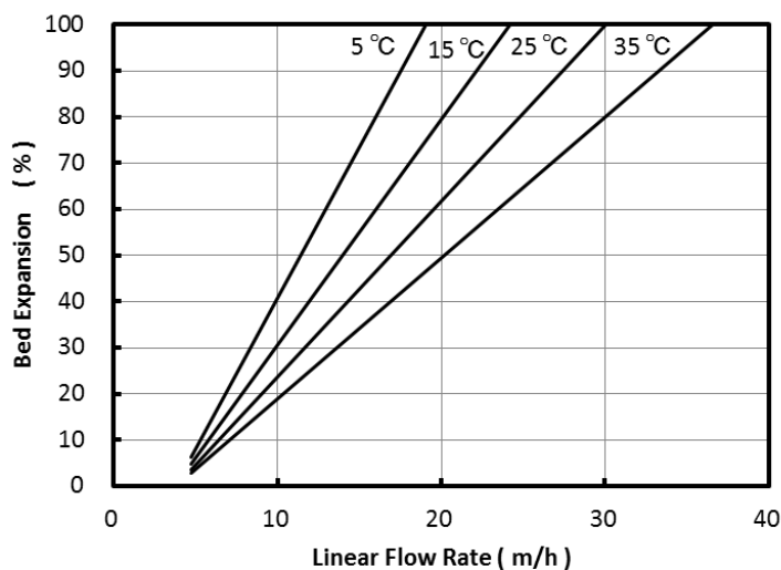
Fig. 2 Bed Expansion of PK220
