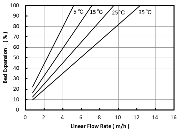
Fig. 2 Bed Expansion of SA10AL
