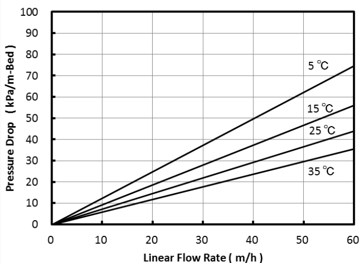
Fig. 1 Pressure Drop of SA10AL
