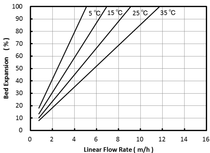
Fig. 2 Bed Expansion of SA12AL
