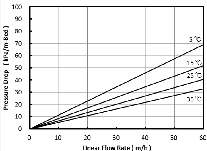
Fig. 1 Pressure Drop of SA12AL
