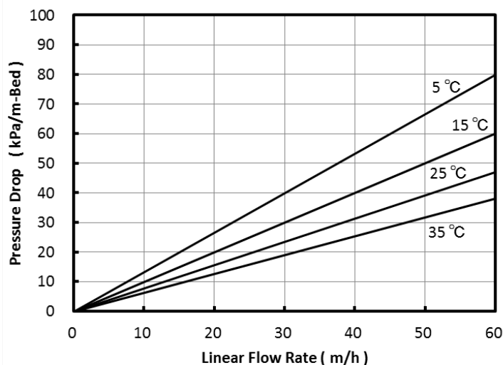
Fig. 1 Pressure Drop of SA20ALL
