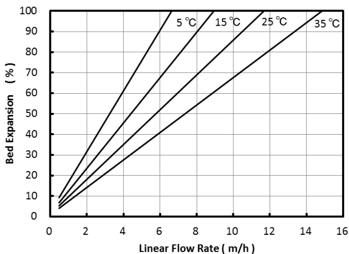
Fig. 2 Bed Expansion of SA20ALL
