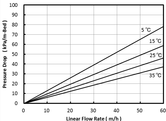
Fig. 1 Pressure Drop of SK112L
