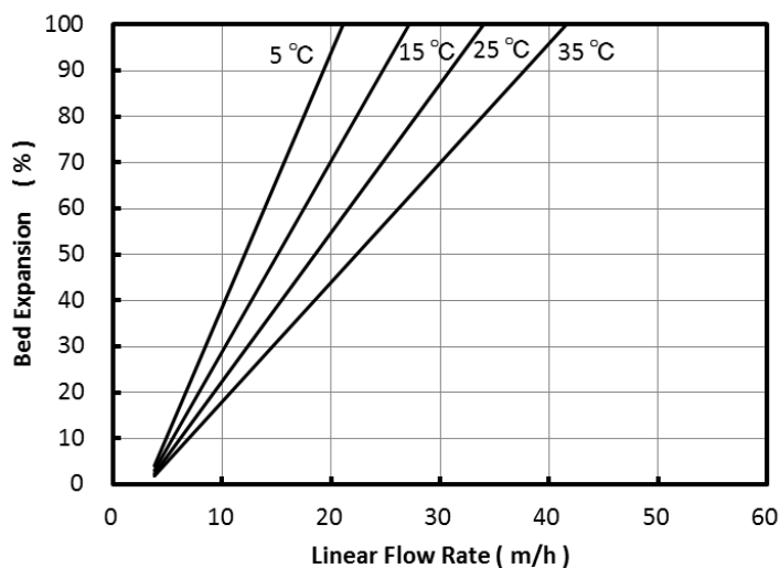
Fig. 2 Bed Expansion of SK112L
