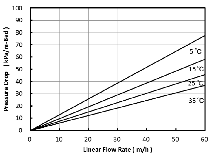
Fig. 1 Pressure Drop of UBK10HUP
