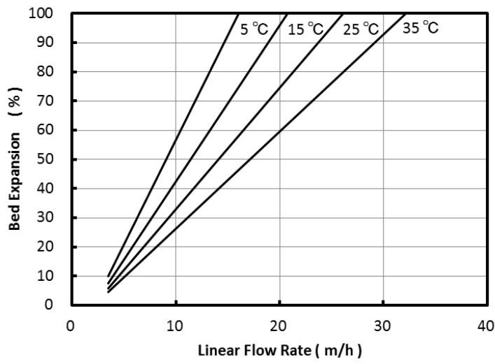
Fig. 2 Bed Expansion of UBK10HUP
