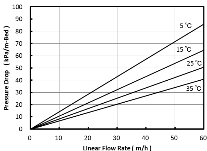
Fig. 1 Pressure Drop of WA20
