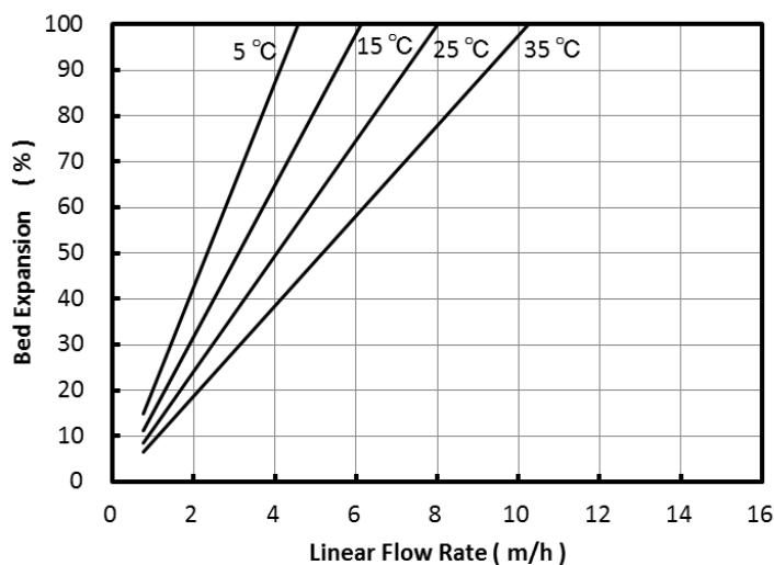
Fig. 2 Bed Expansion of WA20
