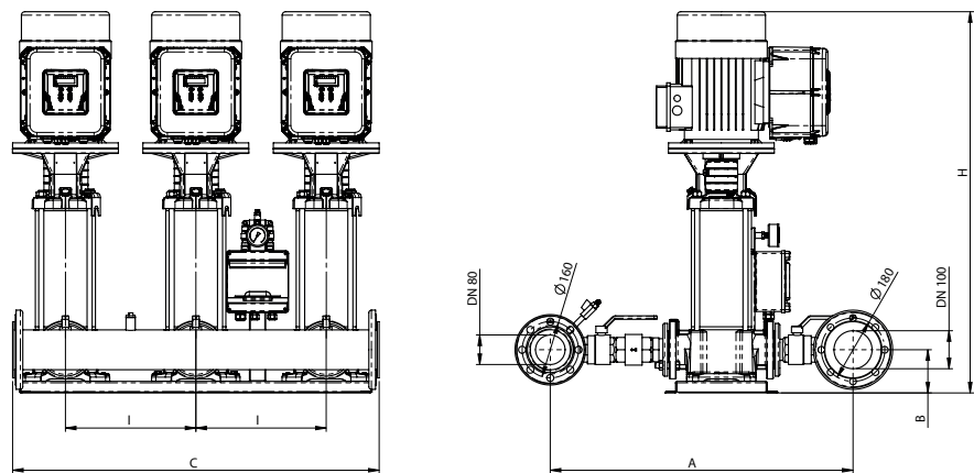
OVERALL DIMENSIONS AND WEIGHTS
