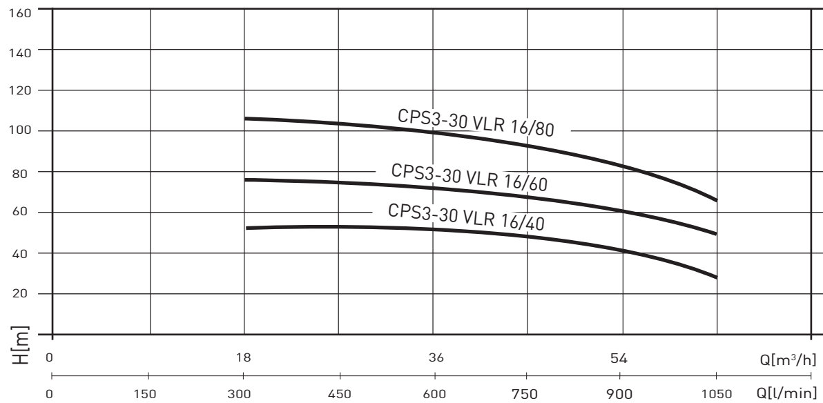
HYDRAULIC PERFORMANCE
