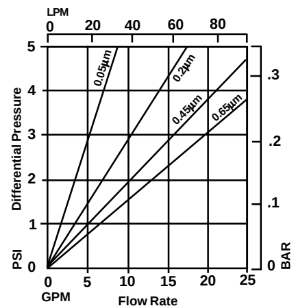
Polyethersulfone Cartridges: Flow rate vs. DP for a 1 cps liquid @ 73°F (23°C)**
