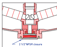
DETAIL 4" THREAD
