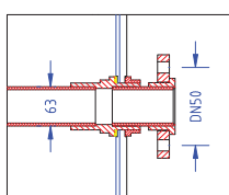
DETAIL SIDE HOLE
