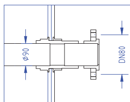
DETAIL DN80
