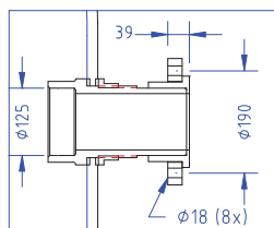
DETAIL SIDE CONNECTION
