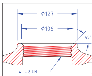
DETAIL 4" THREAD
