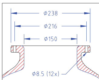
DETAIL 6" FLANGE
