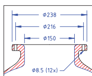
DETAIL 6" FLANGE
