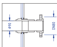
DETAIL DN80
