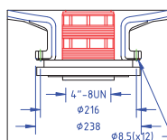
DETAIL 6" TOP/BTM FLANGE
