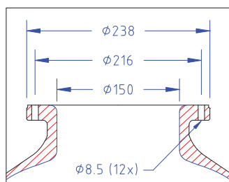
DETAIL 6" FLANGE
