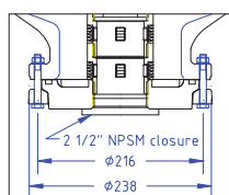
DETAIL 6" FLANGE
