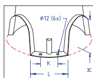
DETAIL BASE
