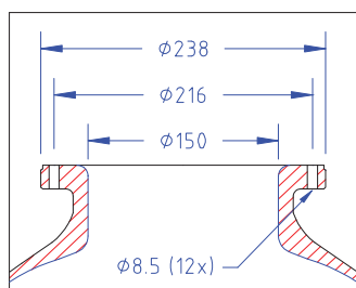
DETAIL 6" FLANGE
