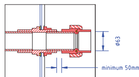
DETAIL SIDE HOLE
