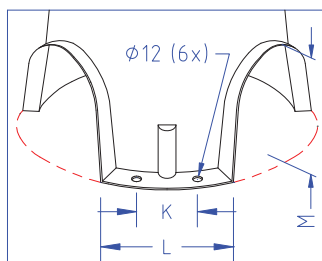
DETAIL BASE
