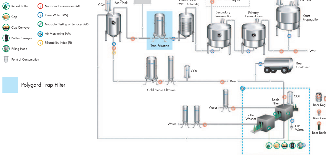
Figure 1. During beer processing, the Polygard Trap Filters are used as prefilters to remove diatomaceous earth from beer and protect the final filter to ensure long filter life.
