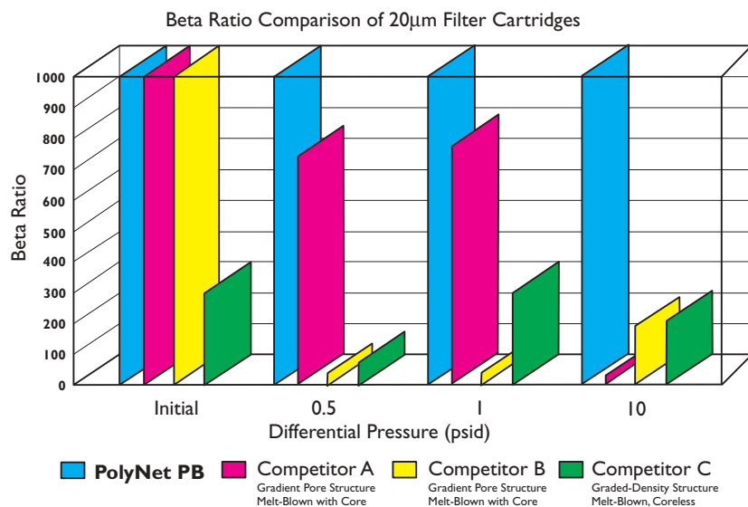
Graph 2. - Beta Ratios demonstrate the PolyNet filter's ability to perform consistently throughout its life
